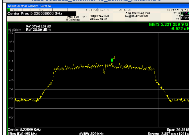
In-Band Reference Level IEEE 802.11a Channel 44 20MHz Antenna 0
