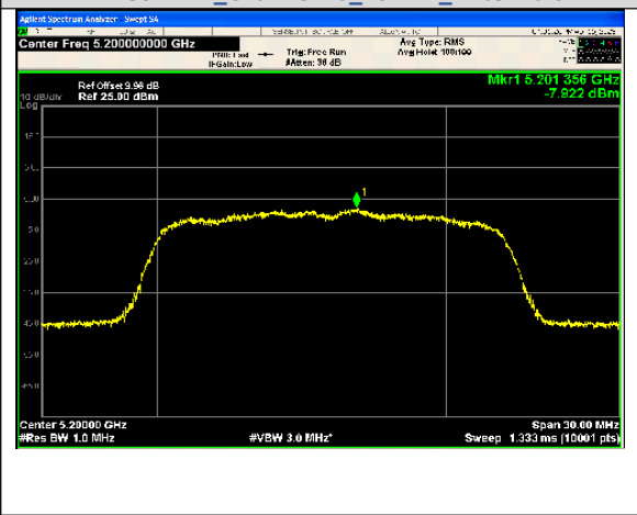
IEEE 802.11ac_Channel 40_20MHz_Antenna 0
