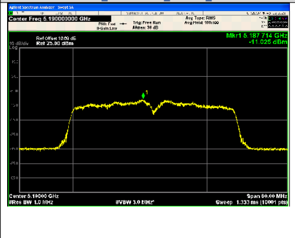
IEEE 802.11ac_Channel 38_40MHz_Antenna 0
