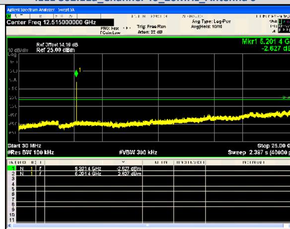
Spurious Emission IEEE 802.11a Channel 40 20MHz Antenna 0
