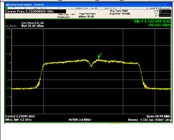
IEEE 802.11n_Channel 46_40MHz_Antenna 0
