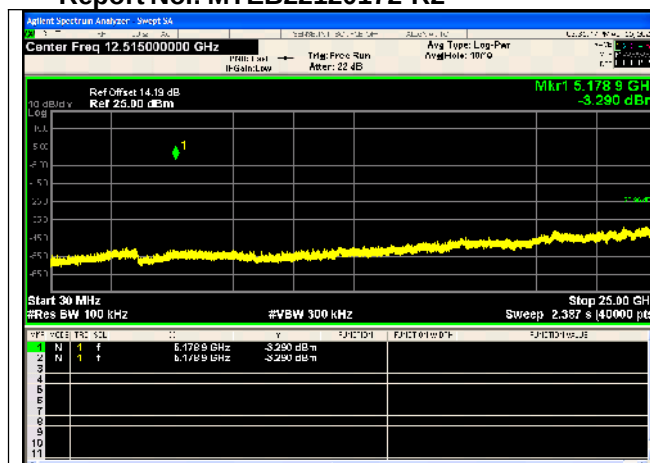
Spurious Emission IEEE 802.11a Channel 36 20MHz Antenna 0
