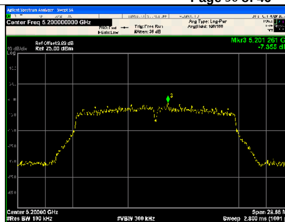
In-Band Reference Level IEEE 802.11a Channel 40 20MHz Antenna 0
