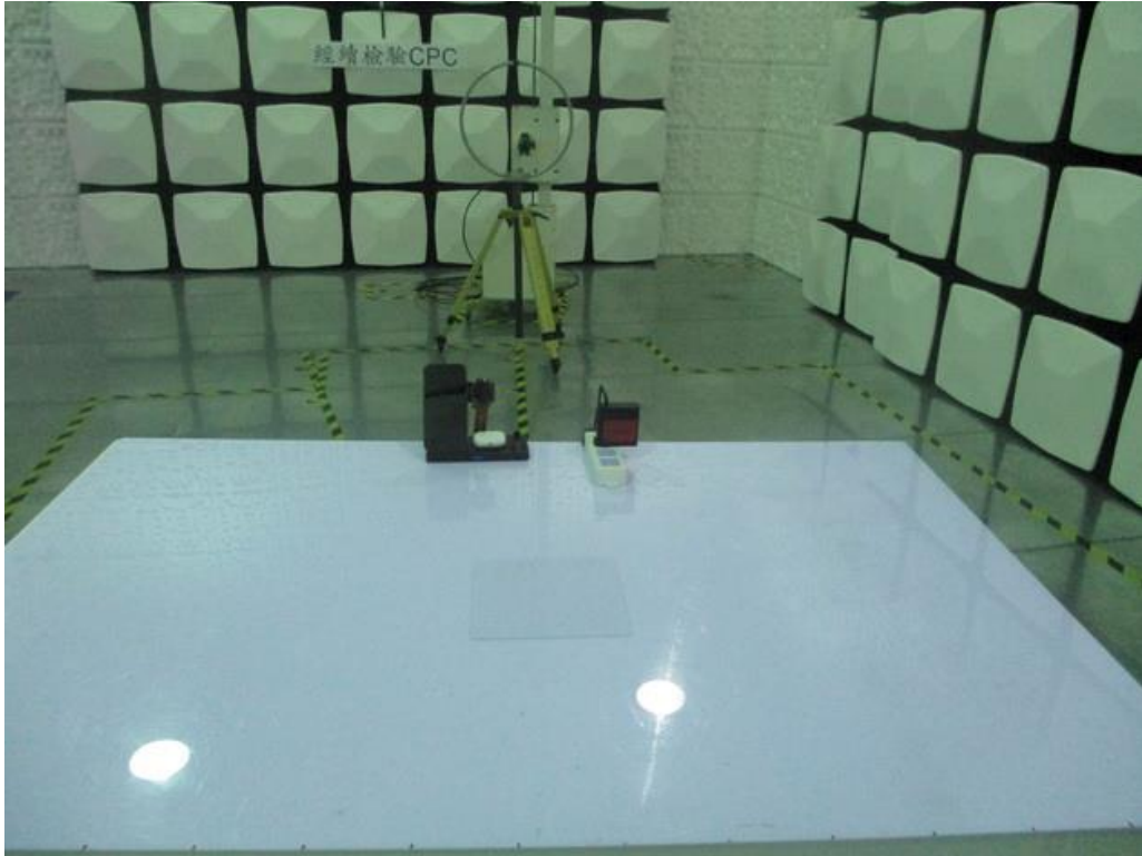
Setup Photo FCC ID: 2A4WMWZC-W5
