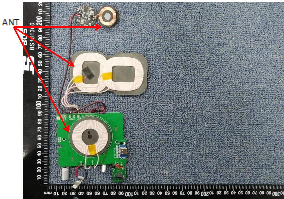
Internal Photo FCC ID: 2A4WMWZC-W5
