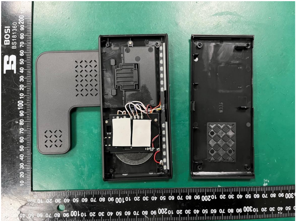
Internal Photo FCC ID: 2A4WMWZC-W336
