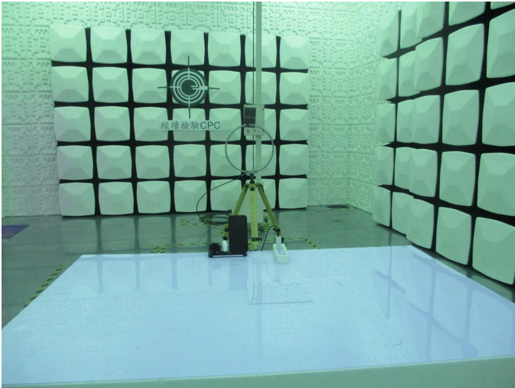
Setup Photo FCC ID: 2A4WMWZC-W320
