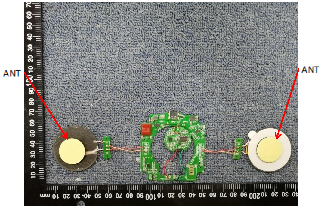
Internal Photo FCC ID: 2A4WMWZC-W312
