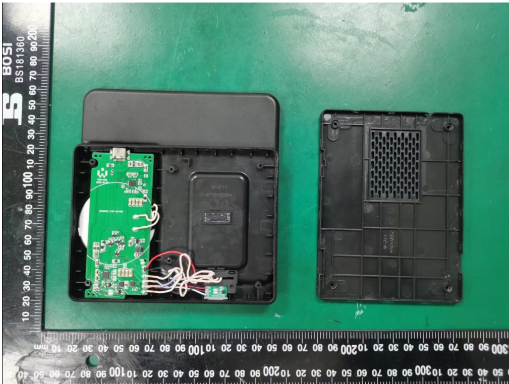
Internal Photo FCC ID: 2A4WMWZC-W311
