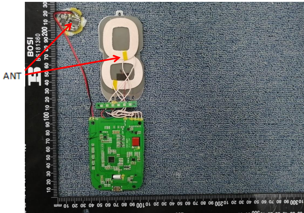
Internal Photo FCC ID: 2A4WMWZC-W306
