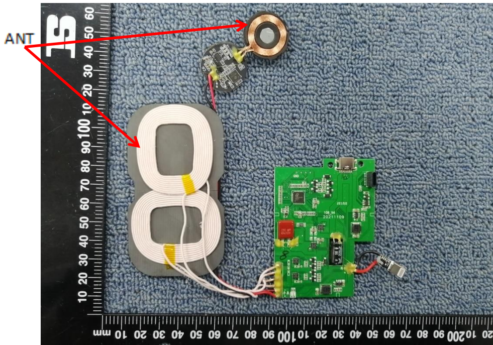
Internal Photo FCC ID: 2A4WMWZC-W3040
