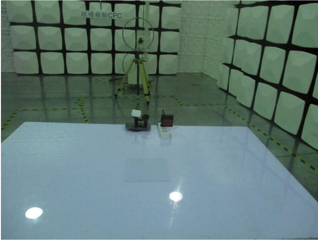
Setup Photo FCC ID: 2A4WMWZC-W3029
