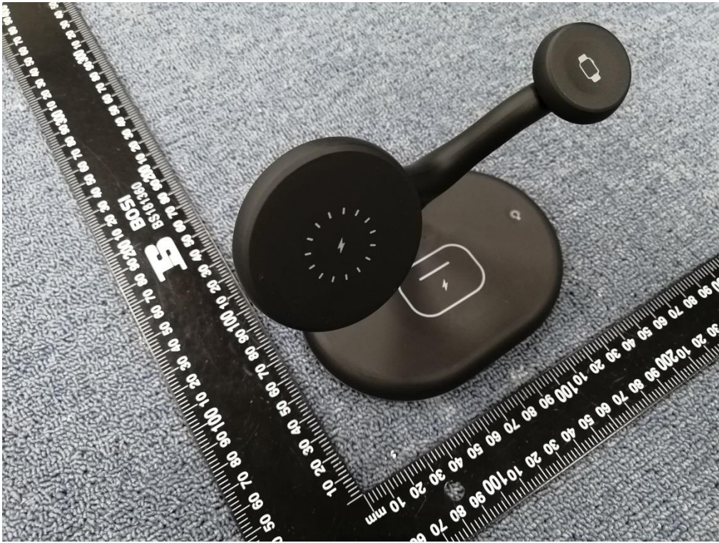
External Photo FCC ID: 2A4WMWZC-W301
