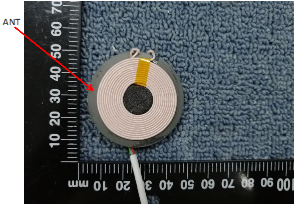
Internal Photo FCC ID: 2A4WMWZC-W207A
