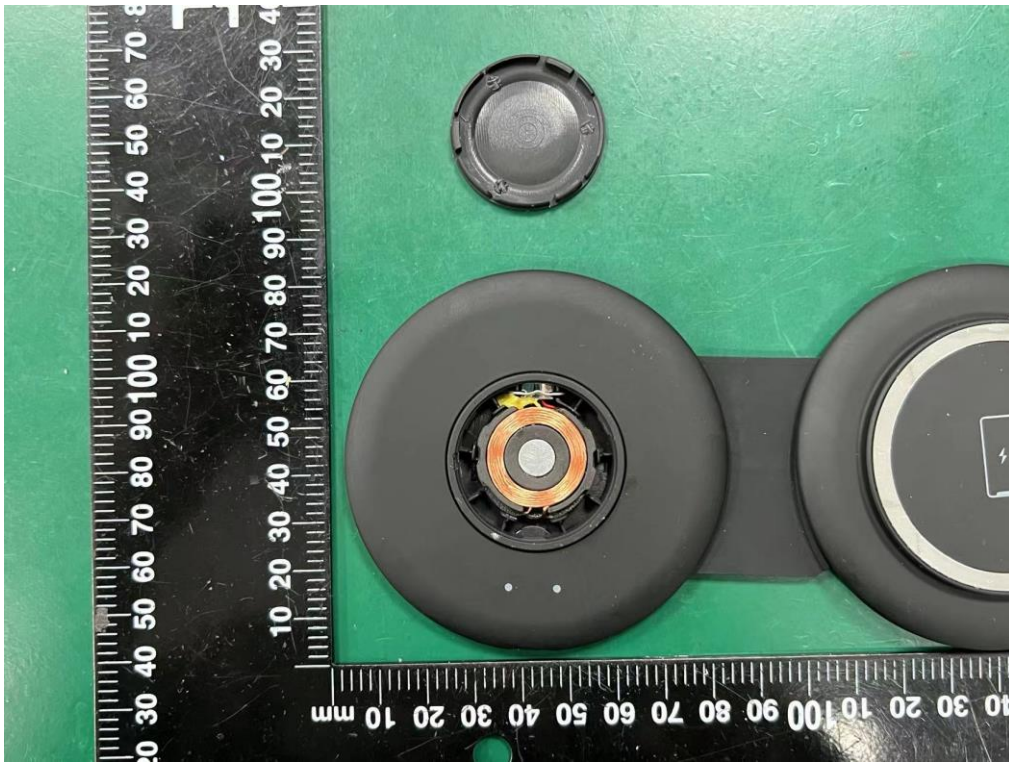
Internal Photo FCC ID: 2A4WMWZC-W203
