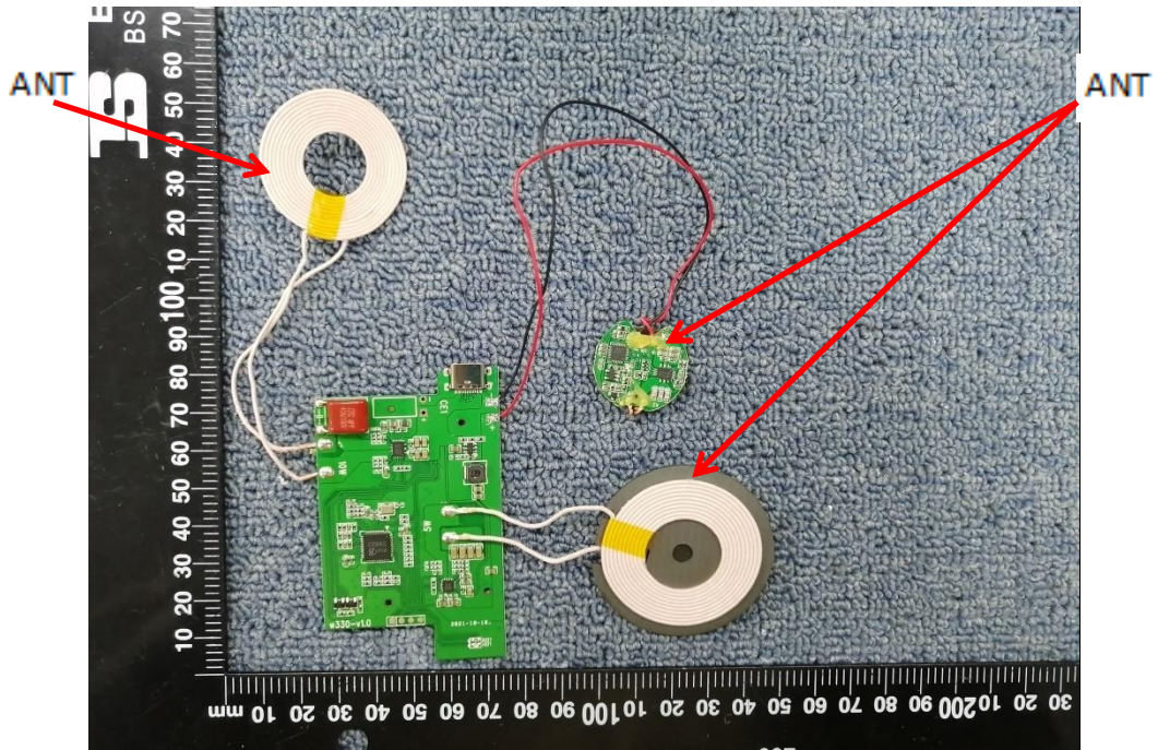
Internal Photo FCC ID: 2A4WMWZC-CW330
