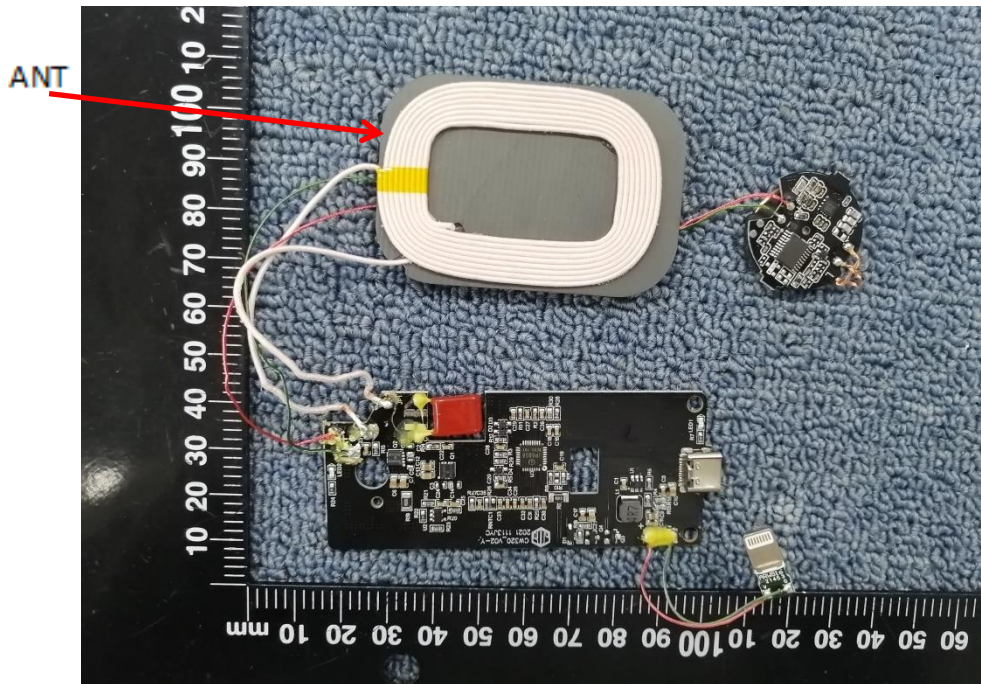
Internal Photo FCC ID: 2A4WMWZC-CW320
