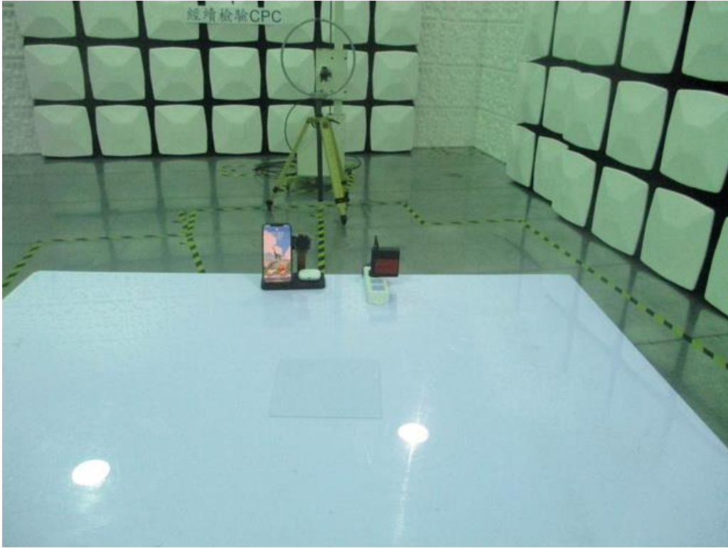
Setup Photo FCC ID: 2A4WMWZC-B16
