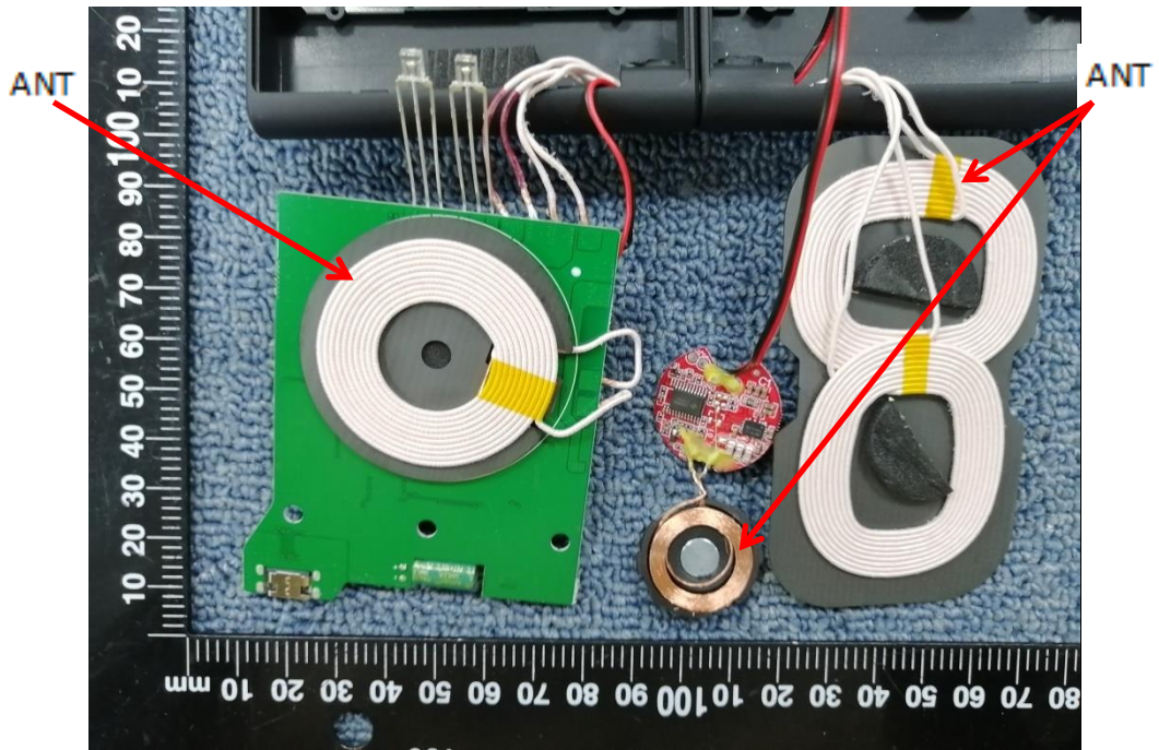
Internal Photo FCC ID: 2A4WMWZC-B16
