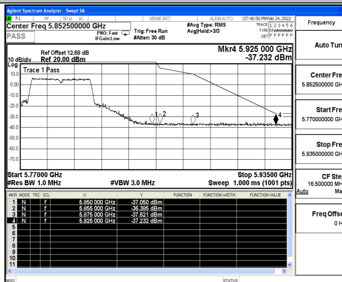
11AC40SISO_Ant_High_5795_Peak
