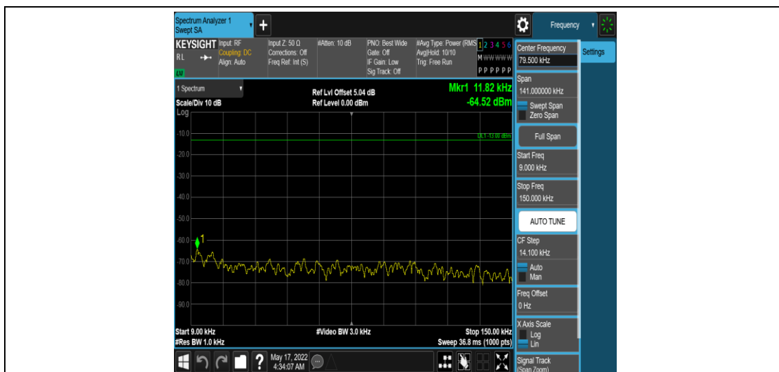
Band12-5MHz-16QAM-23095-1RB#0-Range1:0.009~0.15MHz
