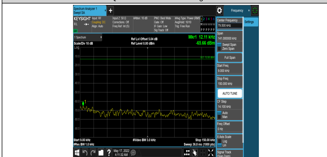
Band12-3MHz-16QAM-23025-1RB#0-Range1:0.009~0.15MHz
