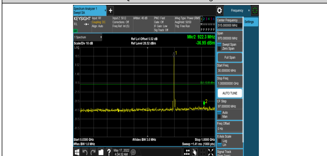
Band12-5MHz-16QAM-23095-1RB#0-Range3:30~1000MHz
