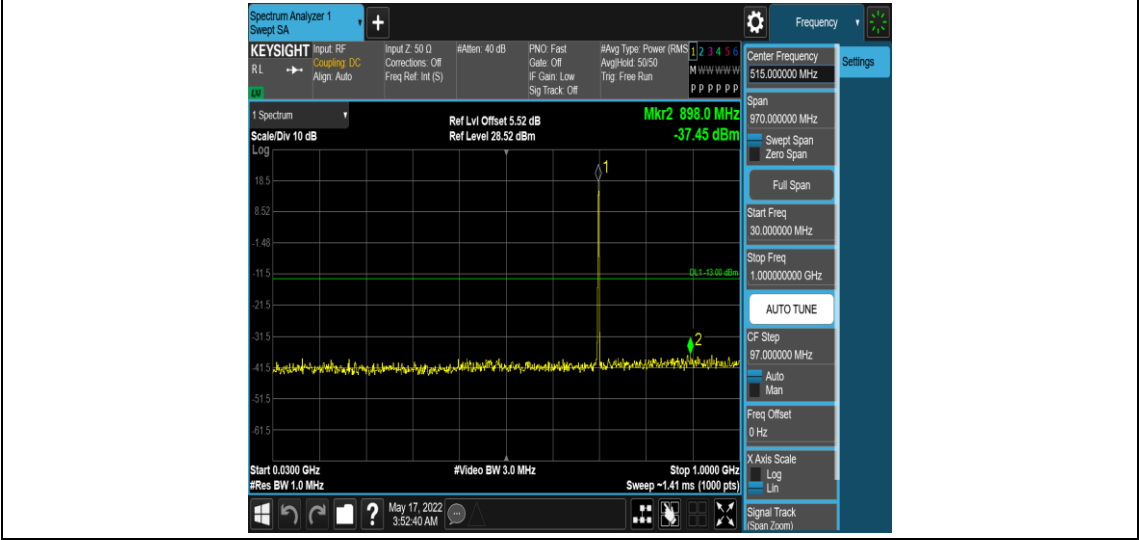
Band12-1.4MHz-QPSK-23095-1RB#0-Range3:30~1000MHz
