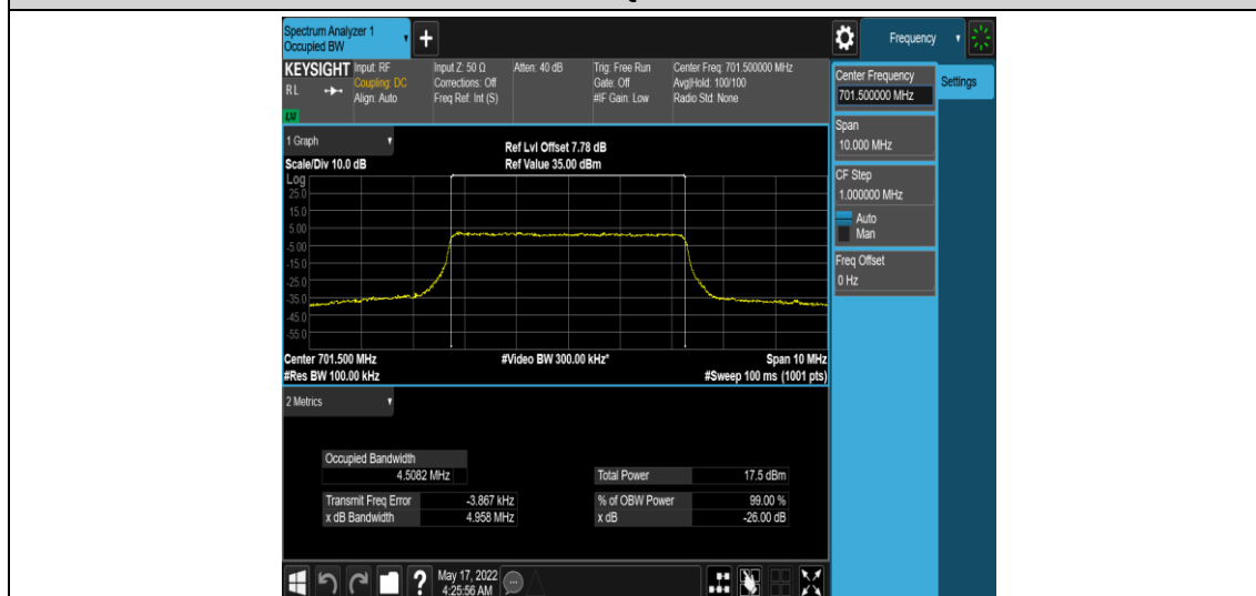
Band12-5MHz-QPSK-23035-25RB#0
