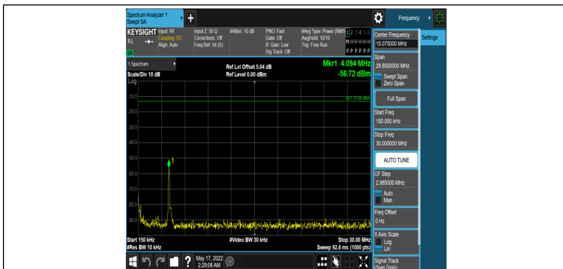
Band7-5MHz-16QAM-21425-1RB#0-Range2:0.15~30MHz
