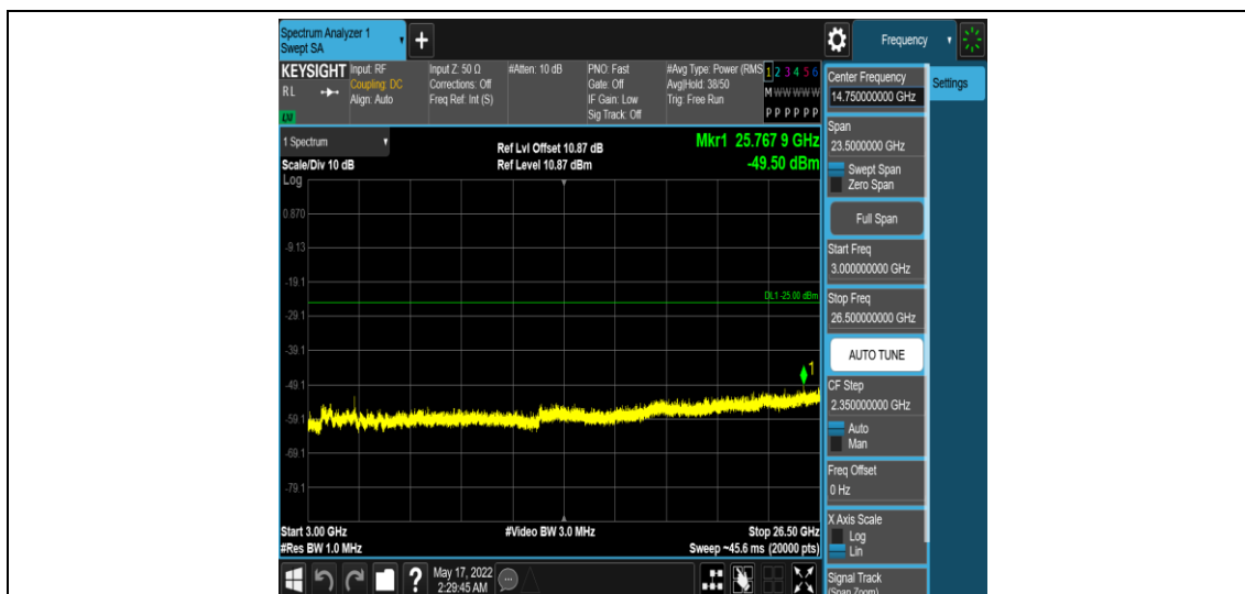
Band7-5MHz-16QAM-21425-1RB#0-Range5:3000~26500MHz
