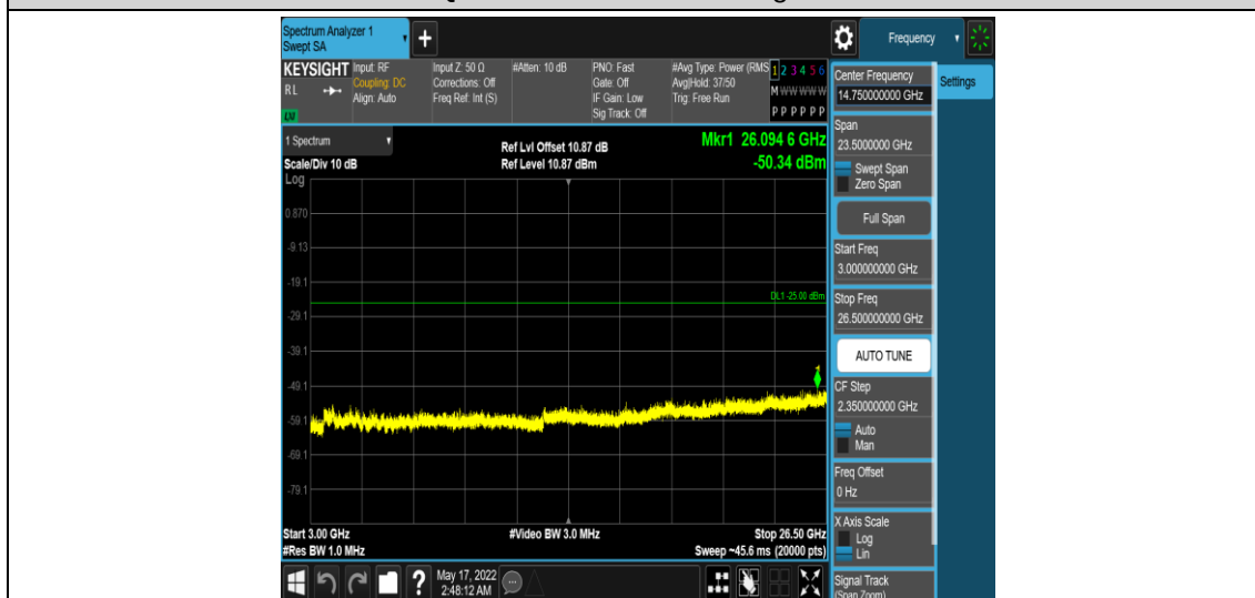
Band7-10MHz-QPSK-21100-1RB#0-Range5:3000~26500MHz
