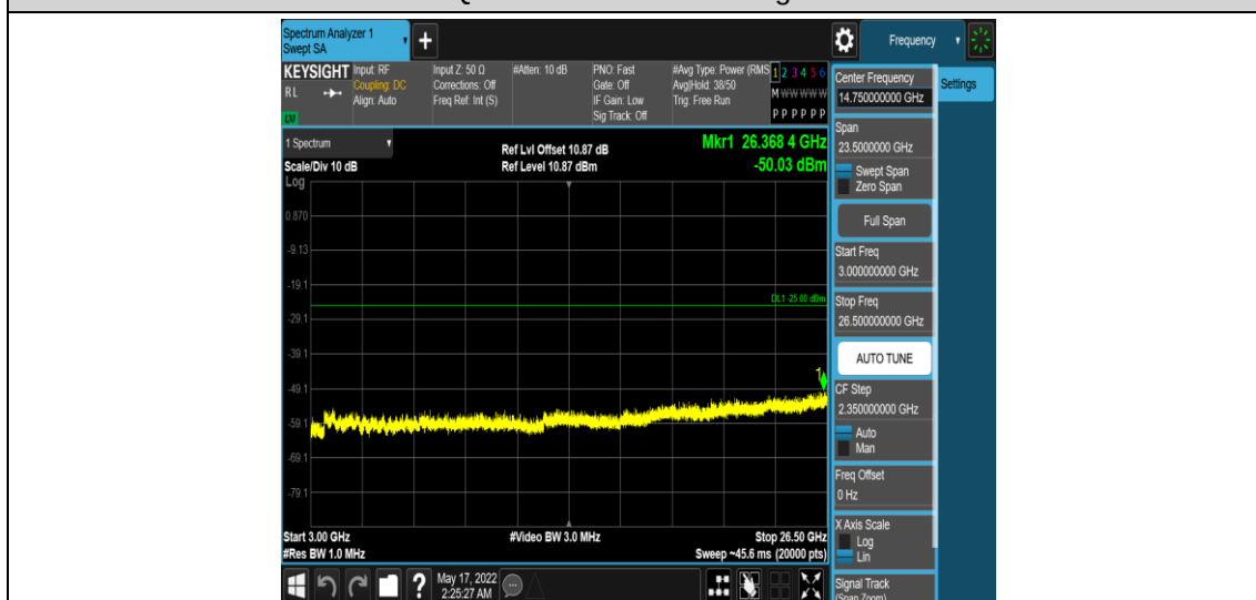
Band7-5MHz-16QAM-20775-1RB#0-Range5:3000~26500MHz
