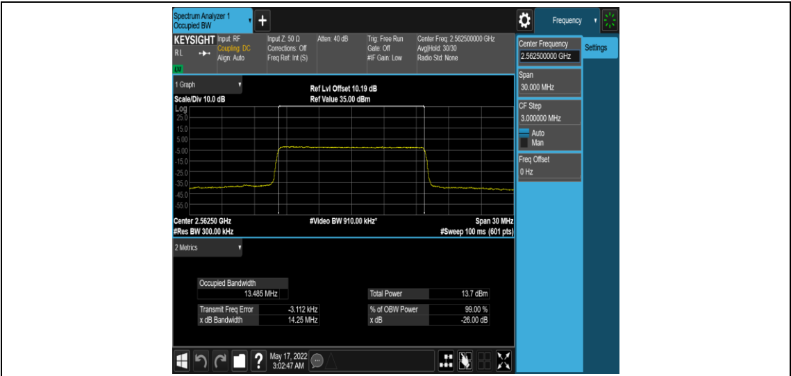
Band7-15MHz-16QAM-21375-75RB#0
