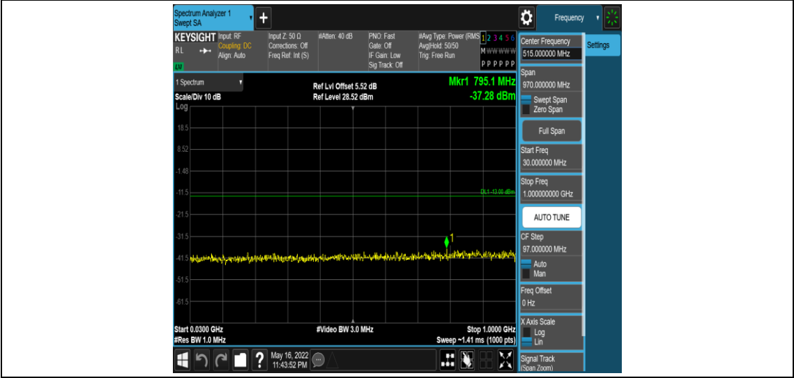
Band4-5MHz-16QAM-20375-1RB#0-Range3:30~1000MHz
