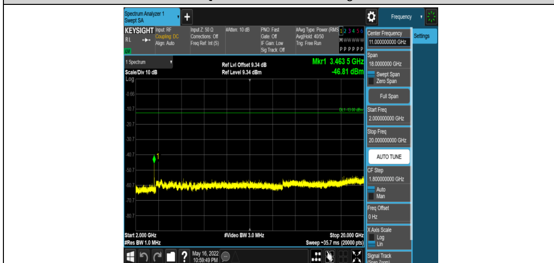
Band4-1.4MHz-16QAM-20175-1RB#0-Range5:2000~20000MHz
