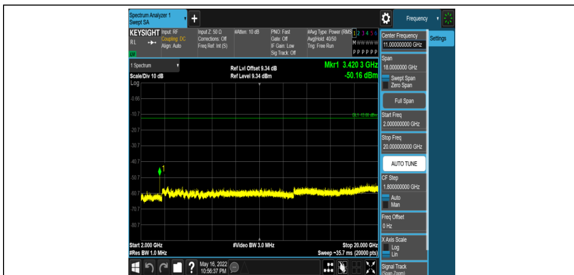
Band4-1.4MHz-QPSK-19957-1RB#0-Range5:2000~20000MHz
