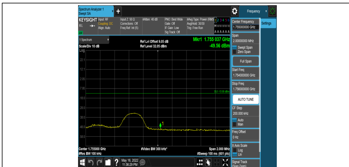
Band4-5MHz-QPSK-20375-1RB#0
