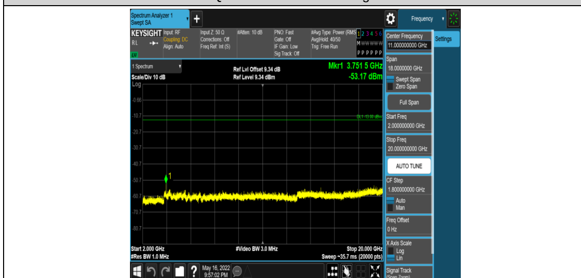
Band2-10MHz-16QAM-18900-1RB#0-Range5:2000~20000MHz
