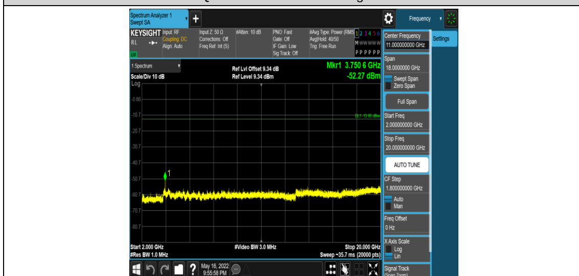
Band2-10MHz-QPSK-18900-1RB#0-Range5:2000~20000MHz
