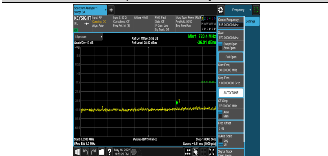
Band2-5MHz-16QAM-18625-1RB#0-Range3:30~1000MHz
