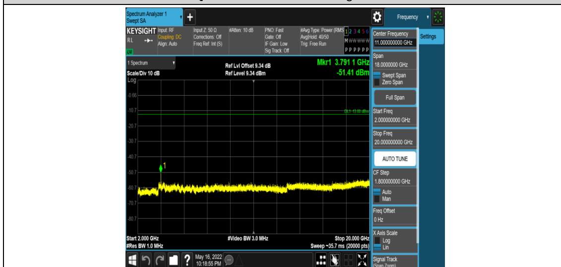
Band2-15MHz-QPSK-19125-1RB#0-Range5:2000~20000MHz
