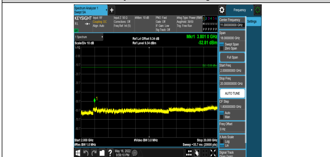
Band2-10MHz-16QAM-19150-1RB#0-Range5:2000~20000MHz
