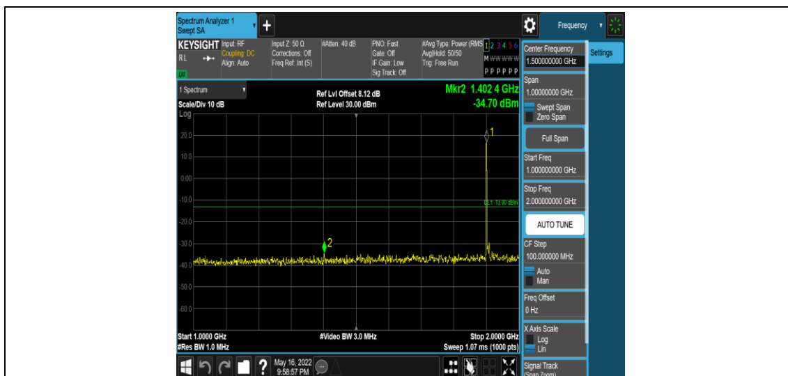
Band2-10MHz-16QAM-19150-1RB#0-Range4:1000~2000MHz
