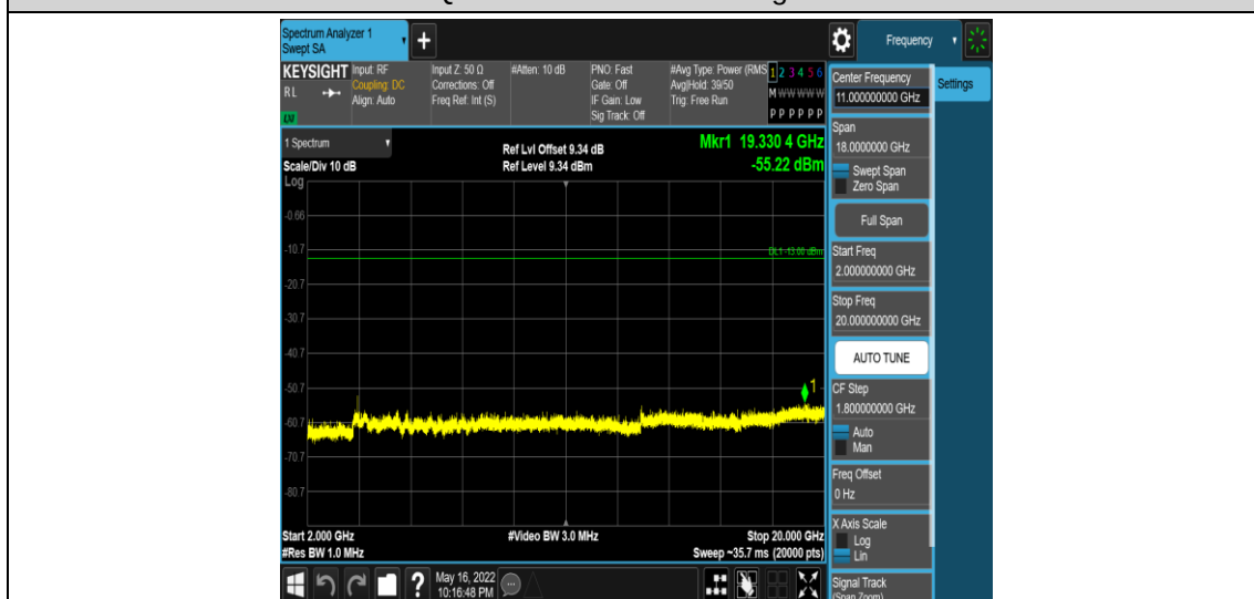
Band2-15MHz-QPSK-18900-1RB#0-Range5:2000~20000MHz
