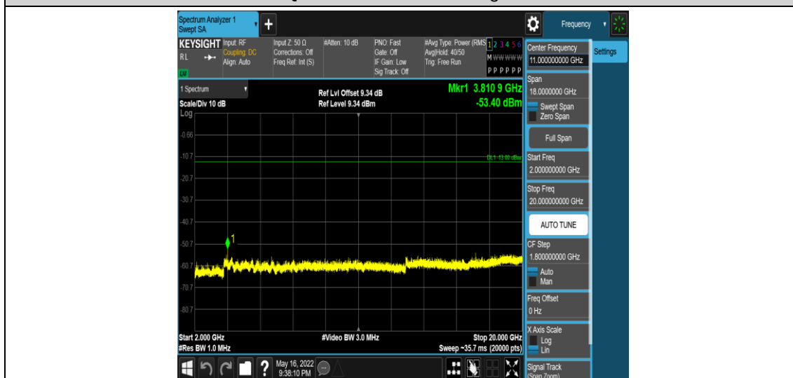
Band2-5MHz-16QAM-19175-1RB#0-Range5:2000~20000MHz
