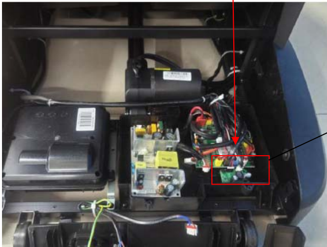
INTERNAL PHOTO OF SAMPLE PCB
