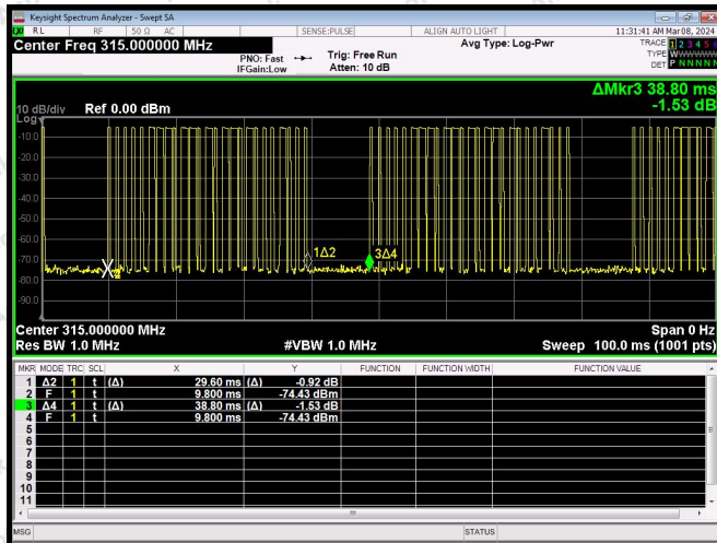
315MHz-T period
