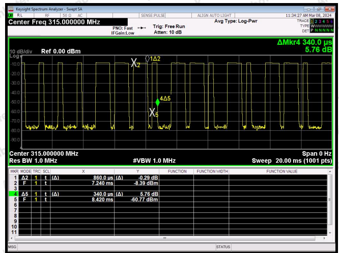
315MHz-T on
