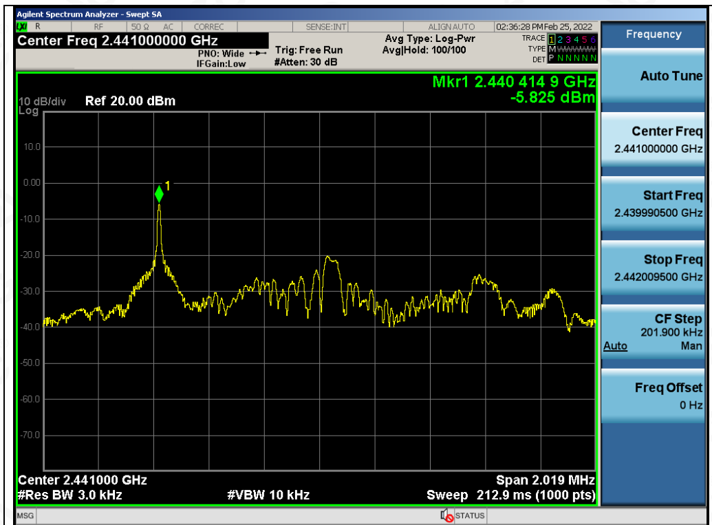
Test_Graph_GFSK_ANT1_2441_2Mbps_PSD
