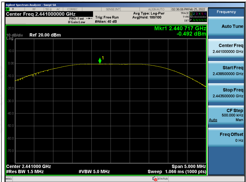
Test_Graph_GFSK_ANT1_2441_Peak Power
