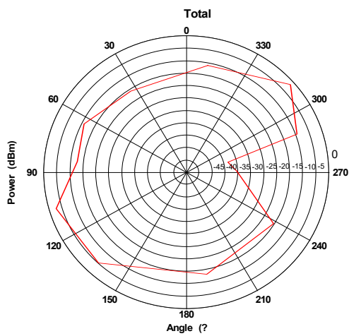
XY Plane at f = 0.434GHz
