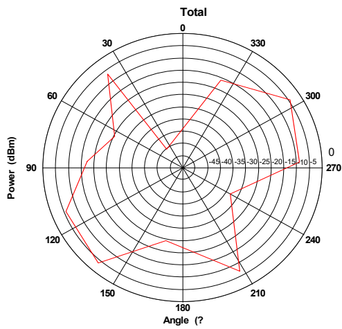
XZ Plane at f = 0.434GHz
