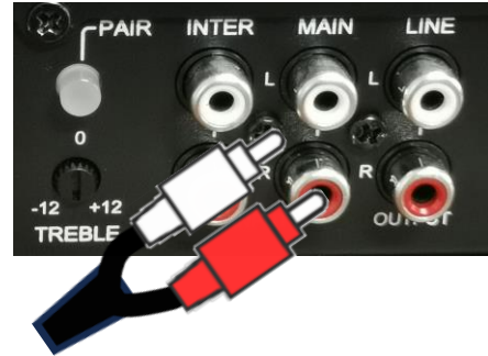
Back Panel RCA Inputs/outputs
