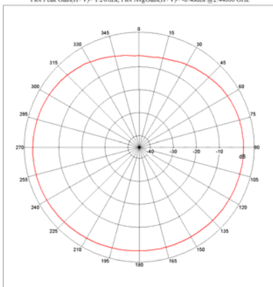
Far-field Power Distribution(H+V) on X-Y Plane Plot Peak Gain(H+V)= 1.20 dB; Plot AvgGain(H+V)= -0.48dB @2.44000 GHz
