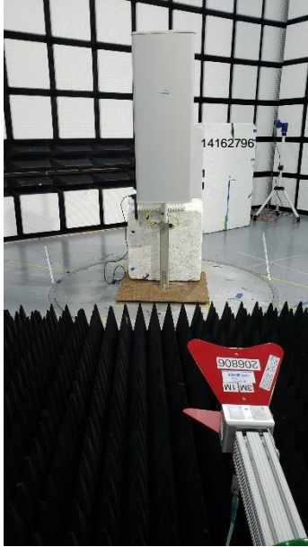
ABOVE 1GHz (FRONT)
