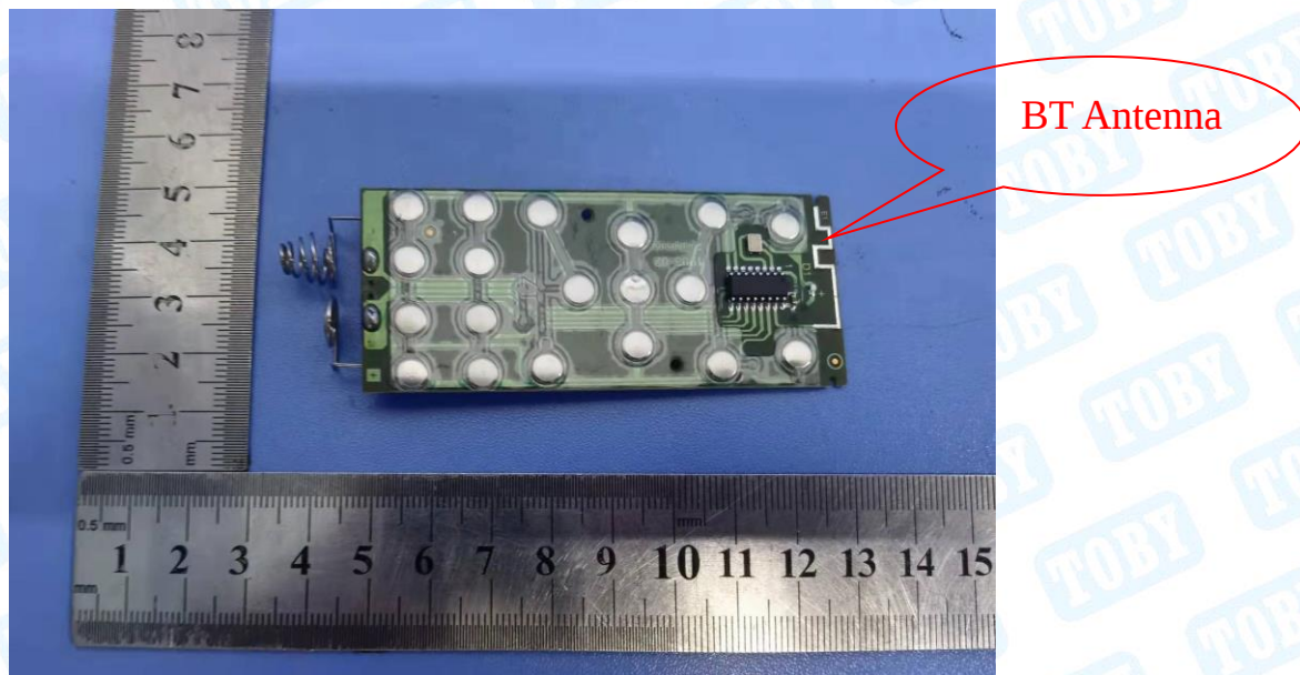
Photo 9 Appearance of PCB
