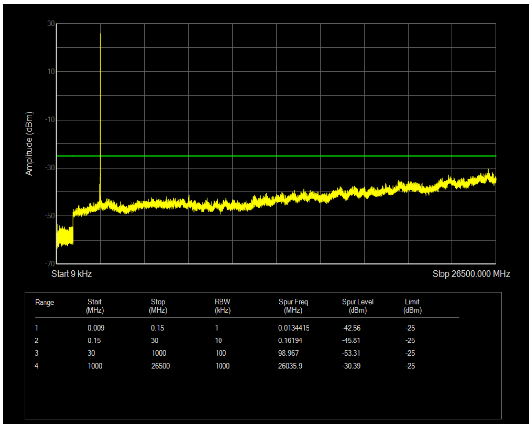
Band41 QAM16 BW=5MHz Channel=41315 RB Size=25 Position=#0
