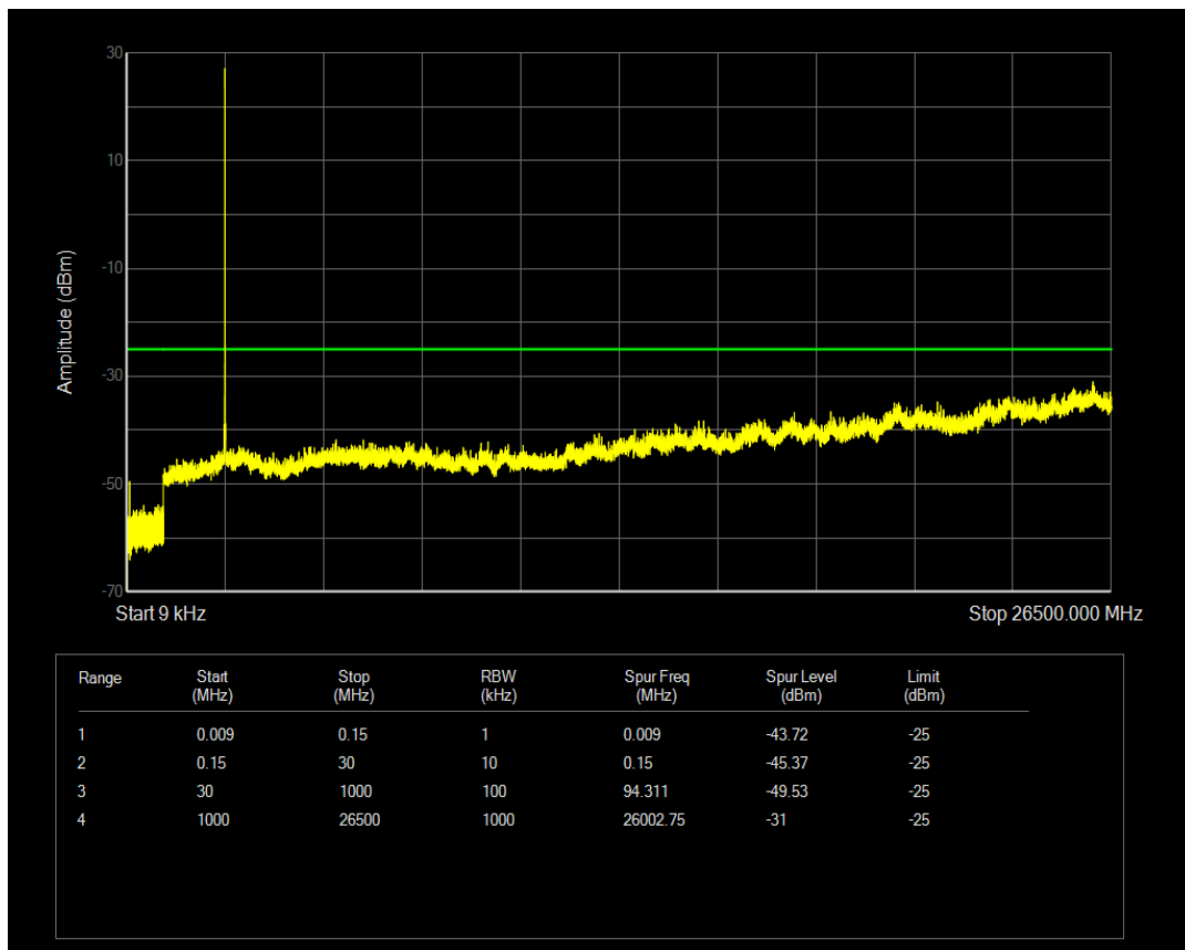
Band41 QPSK BW=10MHz Channel=41290 RB Size=50 Position=#0
