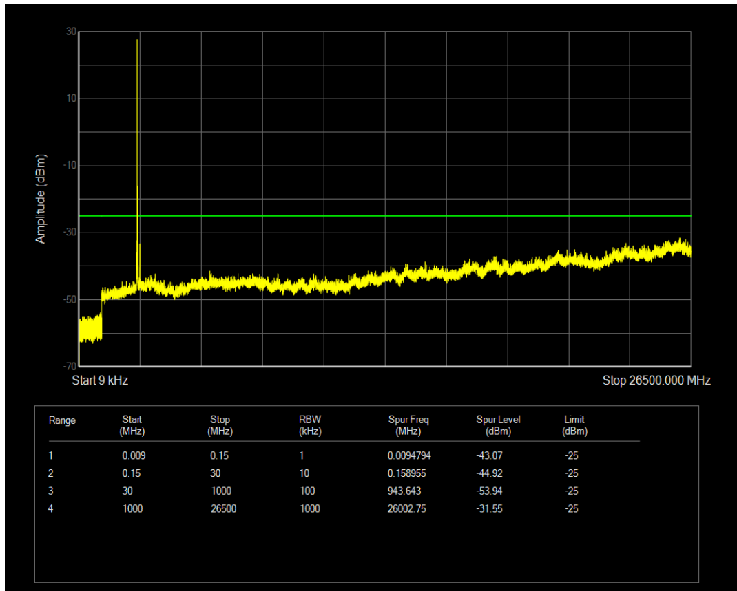
Band41 QAM16 BW=15MHz Channel=41265 RB Size=75 Position=#0
