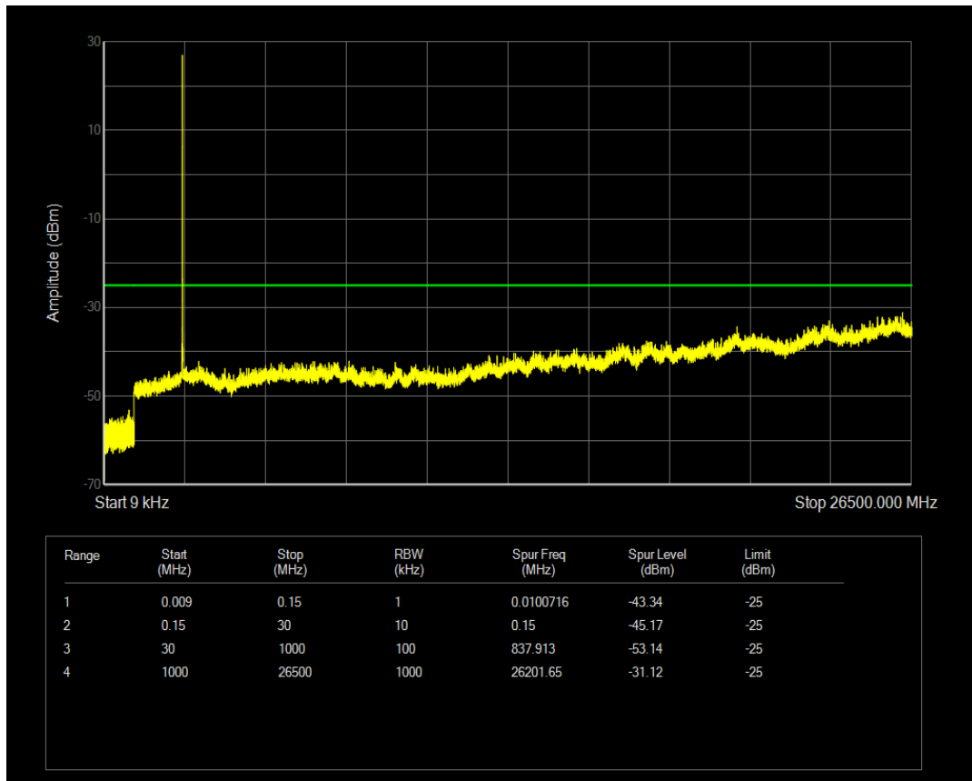
Band41 QPSK BW=10MHz Channel=41290 RB Size=1 Position=#0
