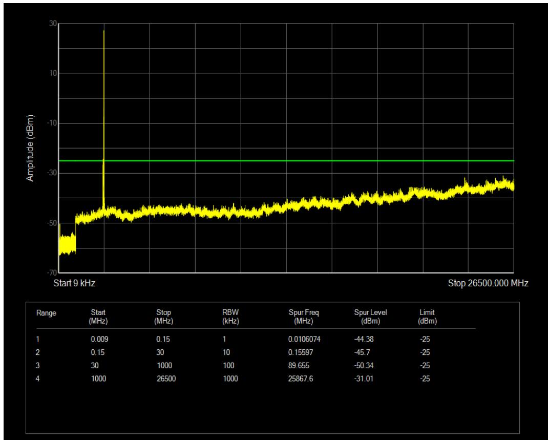
Band41 QAM16 BW=15MHz Channel=41265 RB Size=1 Position=#0
