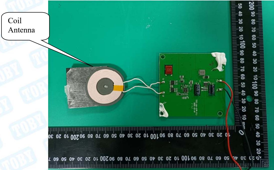
Photo 13 Appearance of PCB
