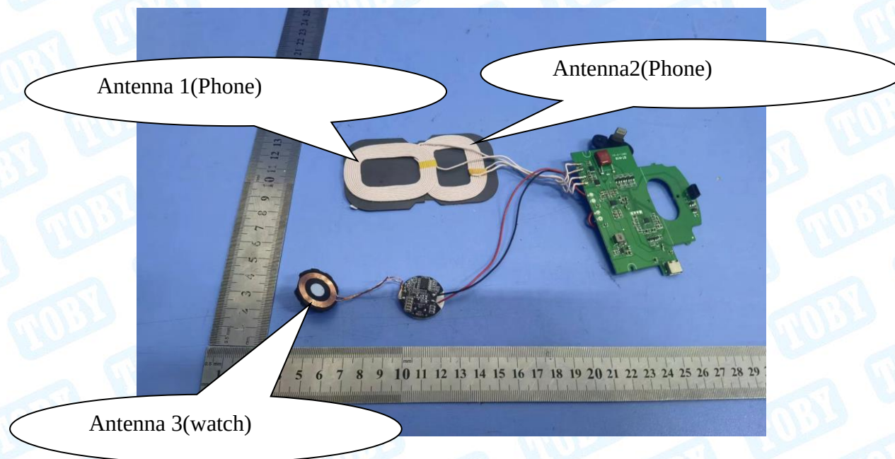
Photo 11 Appearance of PCB
