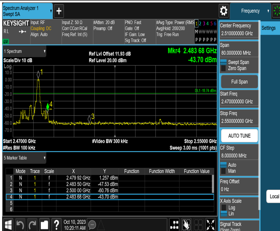
BLE_1M_Ant1_High_2480
