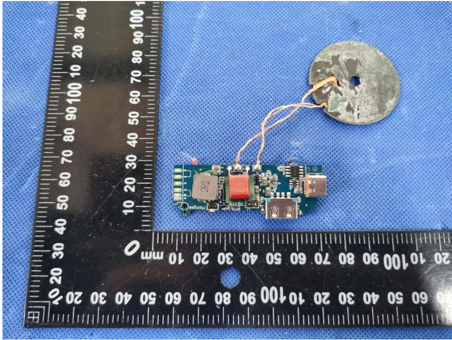
Mobile phone wireless charging ANT
