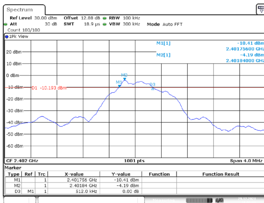
6dB Bandwidth, BLE_1M Low Channel
