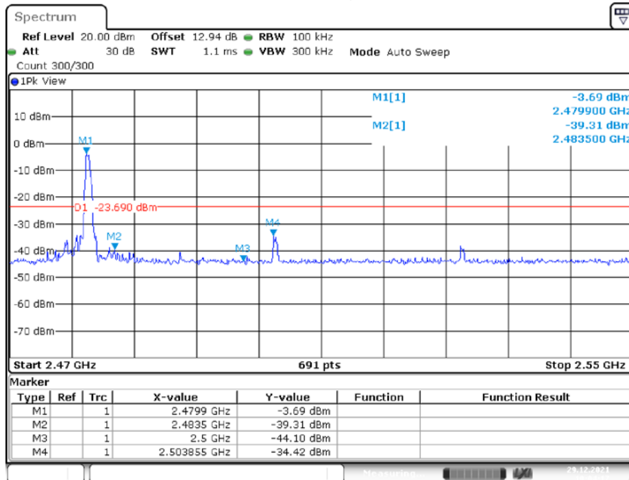
BLE_1M_Ant1_High_2480MHz
