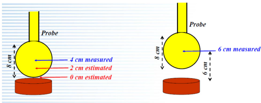
Example of probe measurements in points close to the device surface: estimates compared with measurements at 4 and 6 cm provide validation
