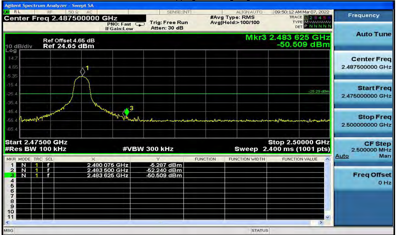
\pi/4 -DQPSK No-hopping Band edge-right side
