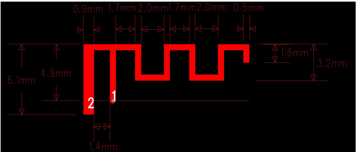
Antenna Dimensions
