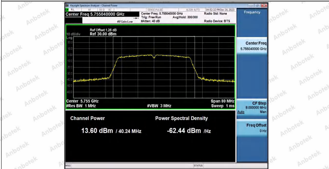
11AC40SISO_WiFi 1_5755
