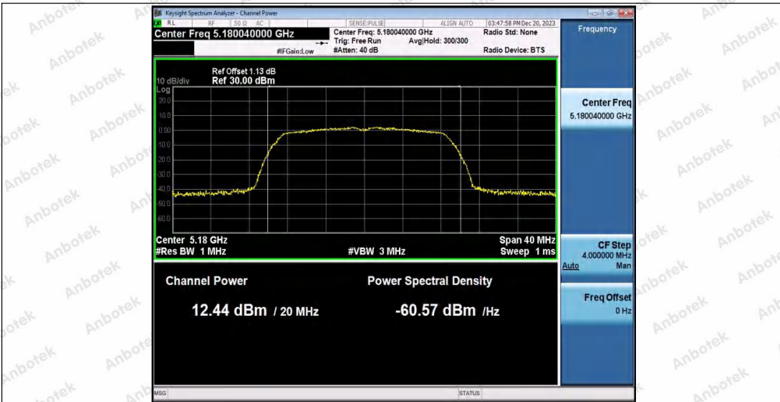
11N20SISO_WiFi 1_5180
