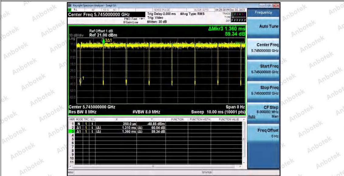
11AC20SISO_WiFi 1_5745
