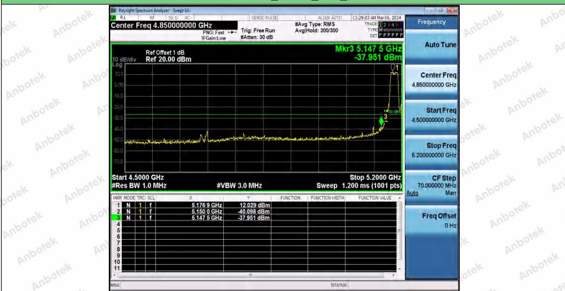
11AC20MIMO_WiFi 1_Low_5180
