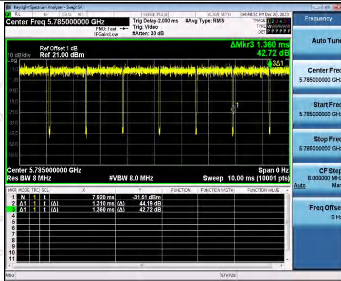
11AC20SISO_WiFi 1_5785
