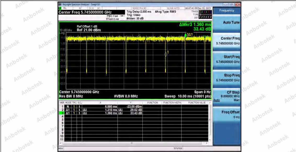
11AC20SISO_WiFi 1_5745
