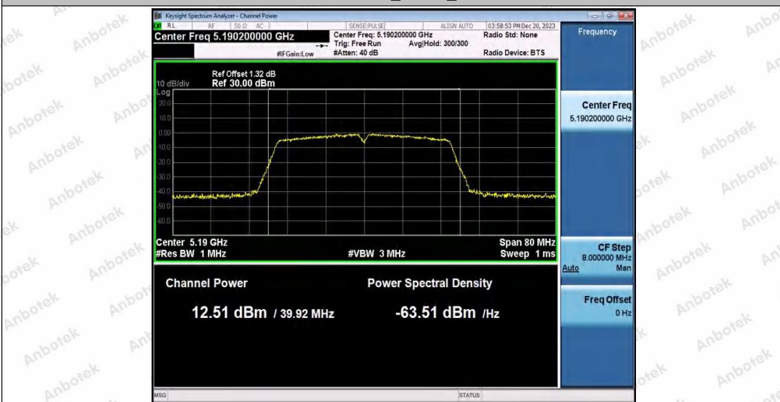
11AC40SISO_WiFi 0_5190
