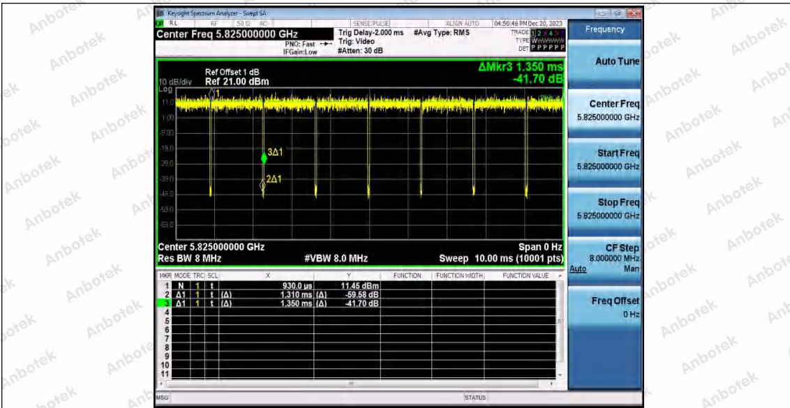
11AC20SISO_WiFi 1_5825
