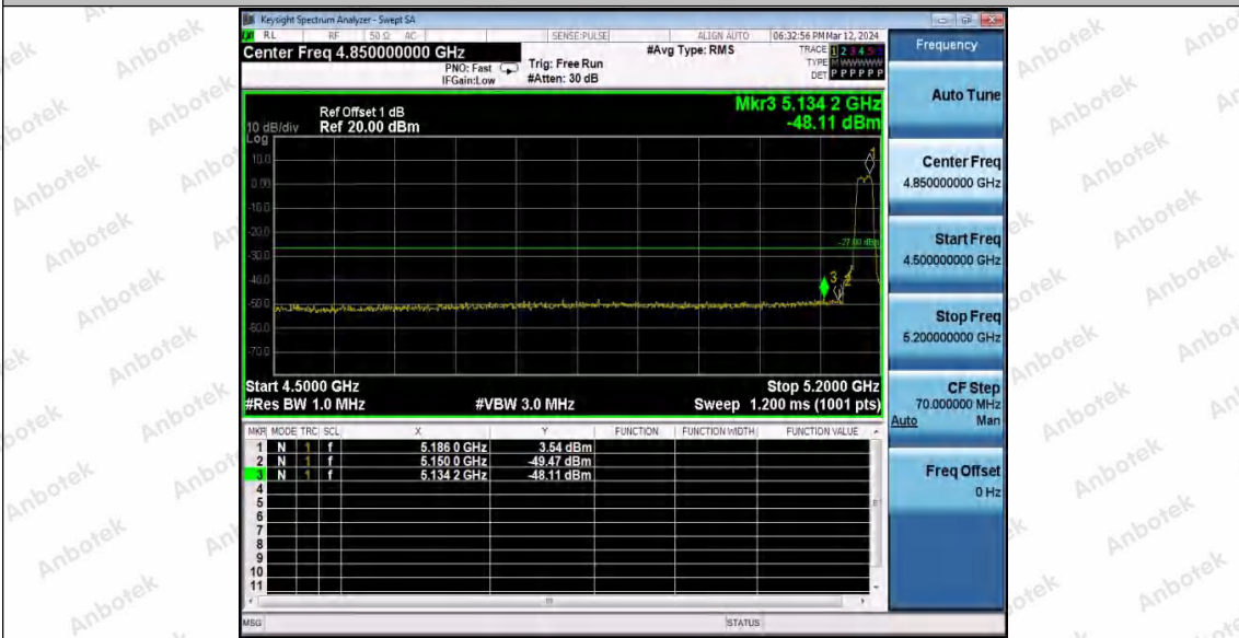
11N20MIMO_WiFi 0_Low_5180
