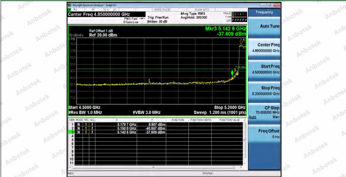
11AC40MIMO_WiFi 1_High_5230
