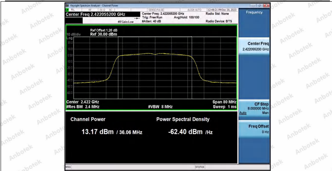
11N40SISO_WiFi 1_2422
