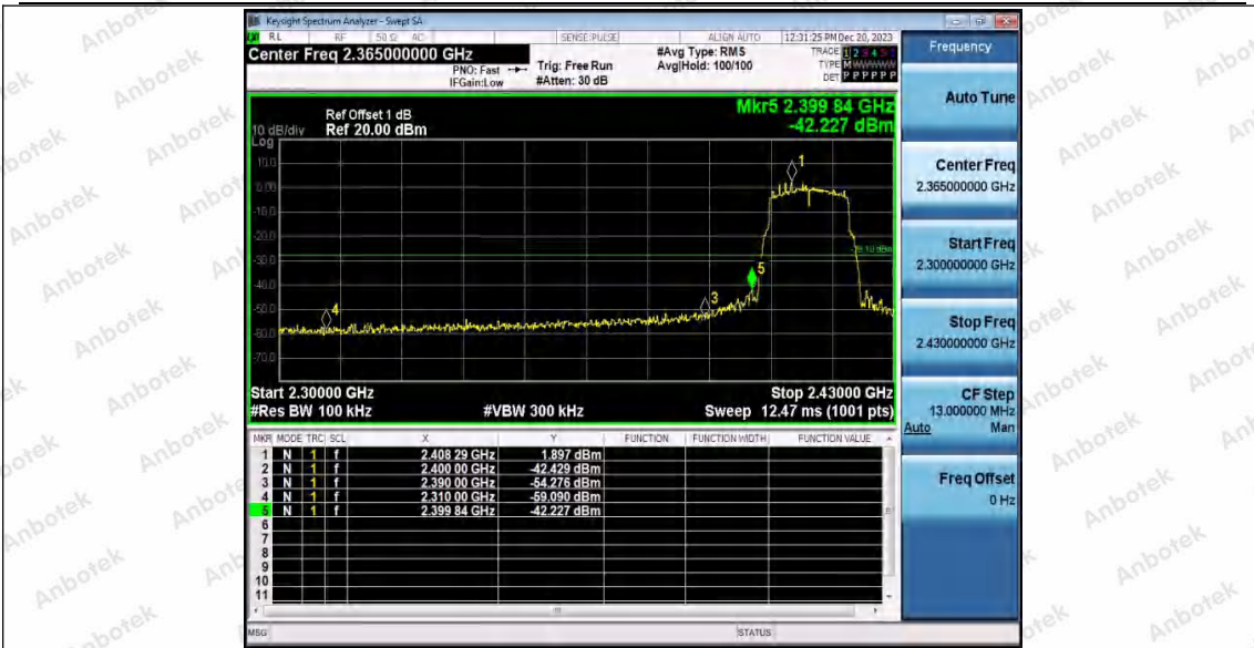
11G_WiFi 1_Low_2412
