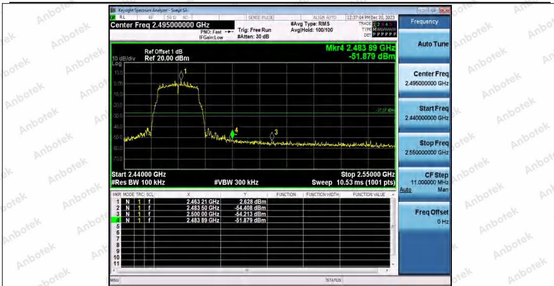
11G_WiFi 1_High_2462
