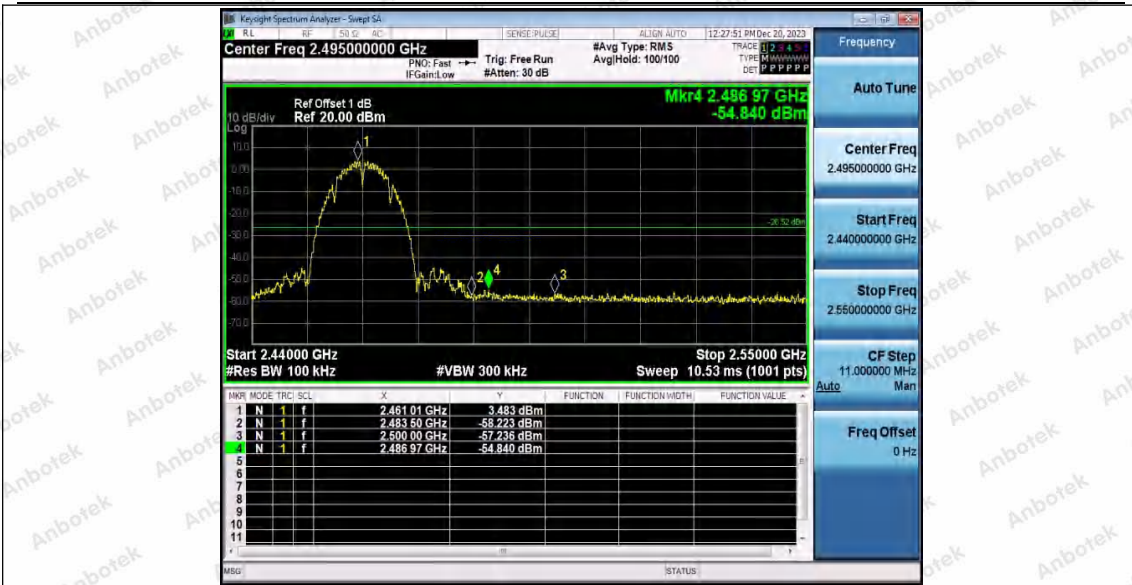
11B_WiFi 1_High_2462
