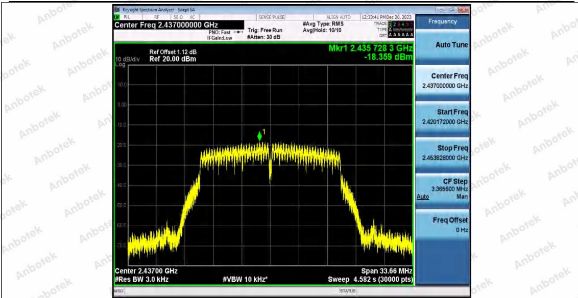
11G_WiFi 1_2437
