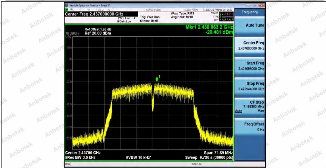
11N40SISO_WiFi 1_2437
