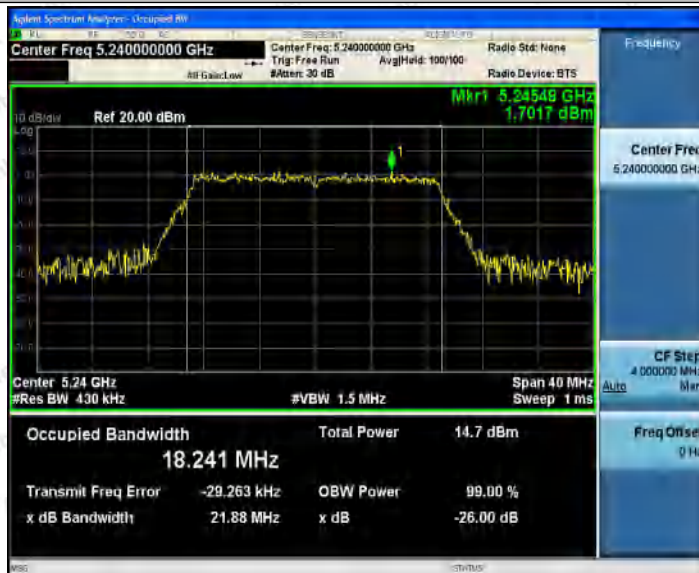
11AC20SISO_Ant2_5240
