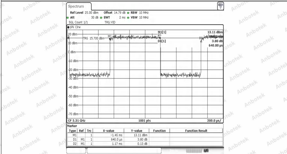
NTNV-11N40SISO-Ant1-5310
