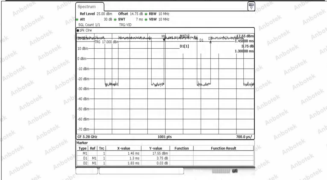
NTNV-11N20SISO-Ant1-5280
