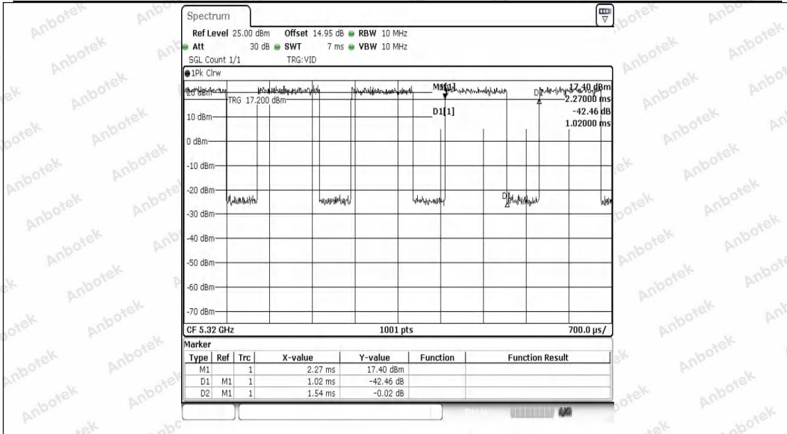
NTNV-11AX20SISO-Ant1-5320
