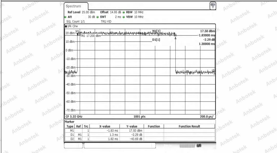
NTNV-11N20SISO-Ant1-5320
