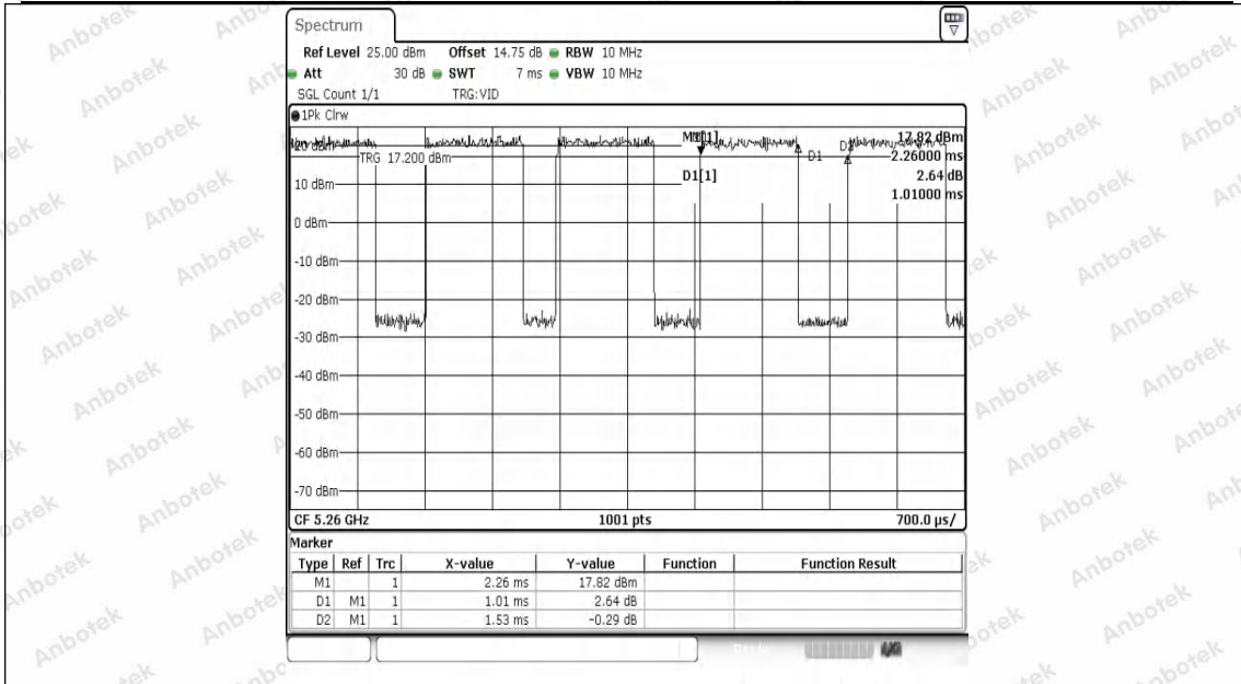
NTNV-11AX20SISO-Ant1-5260
