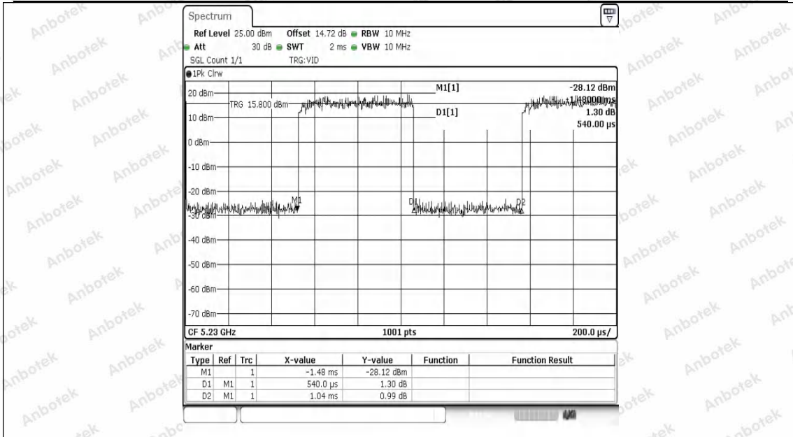
NTNV-11AX40SISO-Ant1-5230
