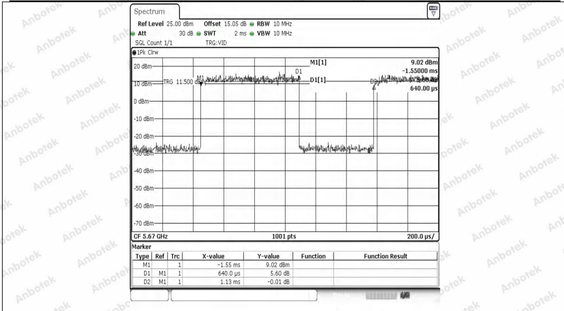
NTNV-11N40SISO-Ant1-5670
