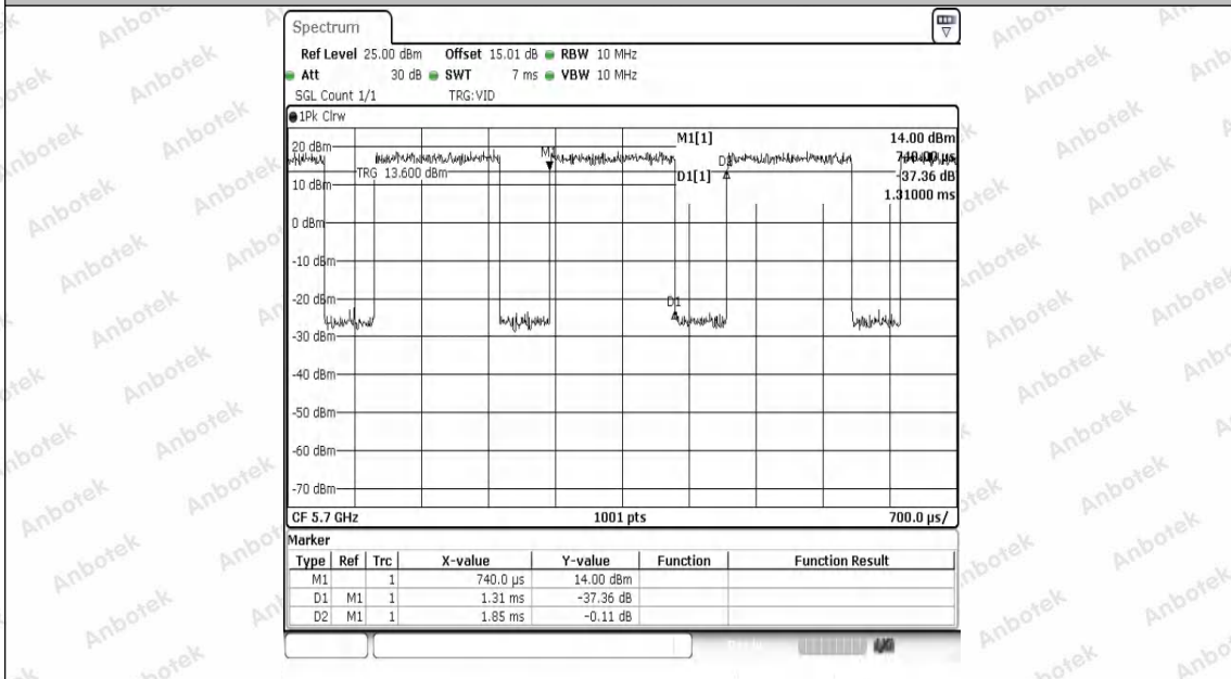
NTNV-11AC20SISO-Ant1-5700
