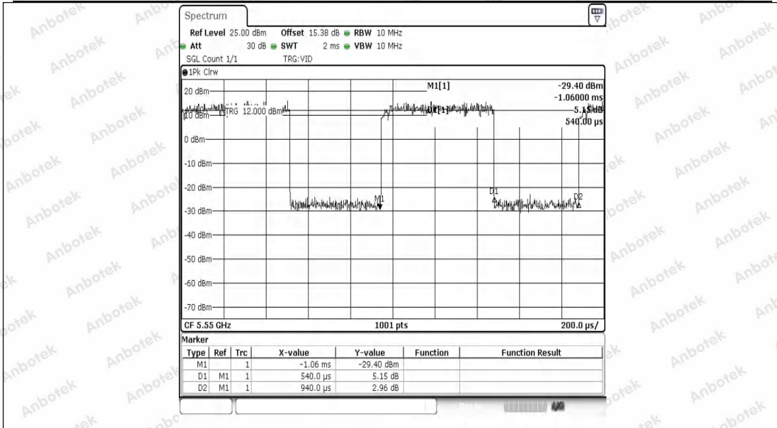
NTNV-11AX40SISO-Ant1-5550
