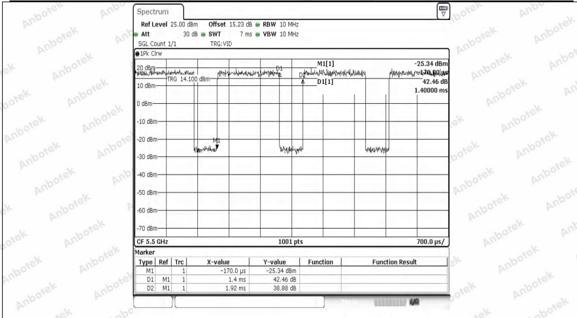
NTNV-11A-Ant1-5500
