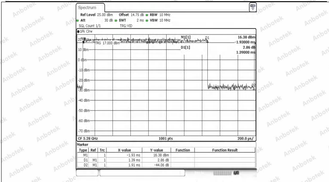
NTVN-11A-Ant1-5280
