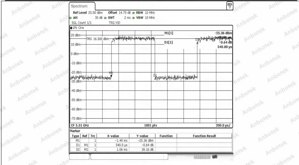
NTVN-11AX40SISO-Ant1-5310
