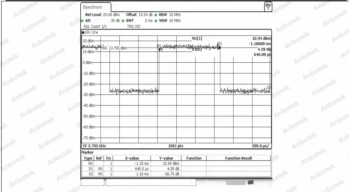
NTNV-11N40SISO-Ant1-5795
