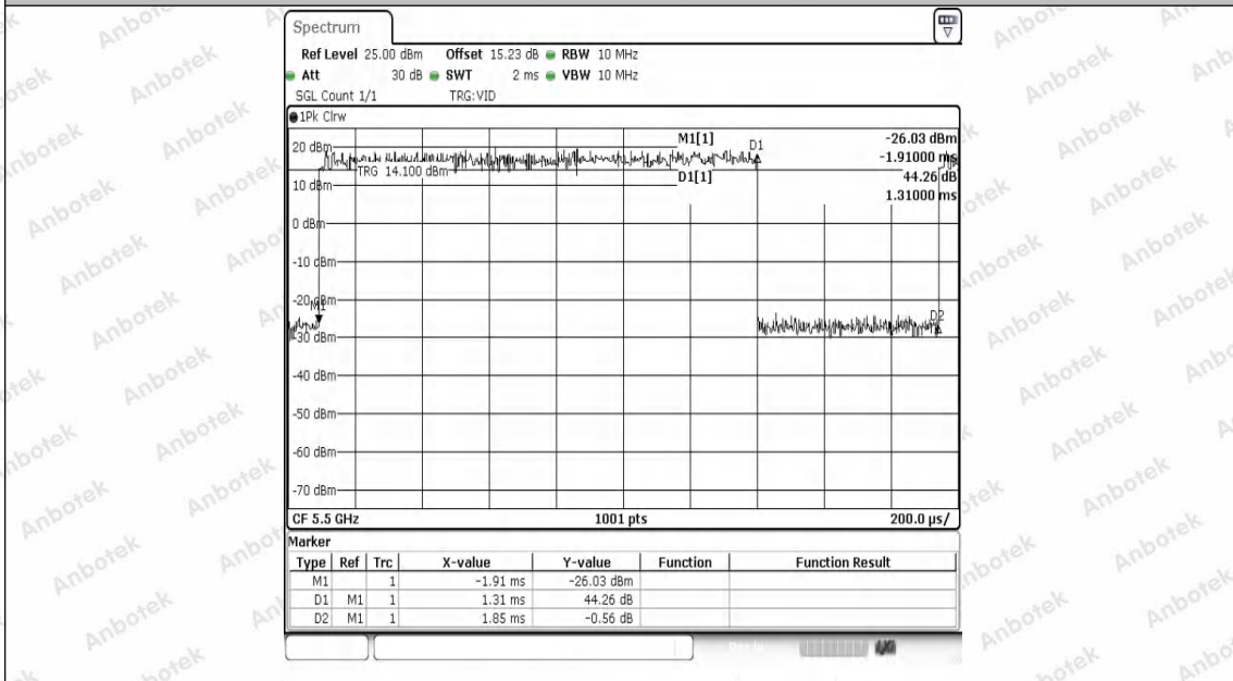
NTVN-11AC20SISO-Ant1-5500
