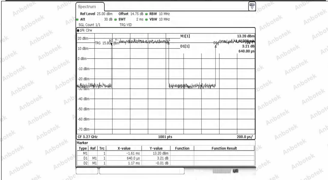
NTNV-11N40SISO-Ant1-5270
