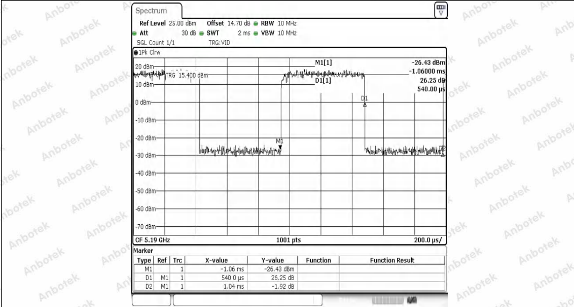
NTNV-11AX40SISO-Ant1-5190
