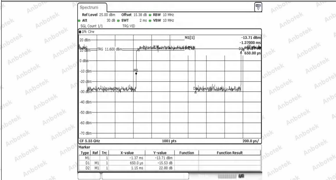
NTNV-11N40SISO-Ant1-5550
