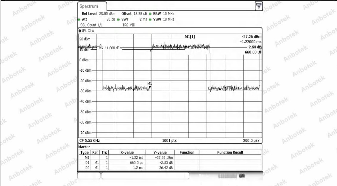
NTNV-11AC40SISO-Ant1-5550
