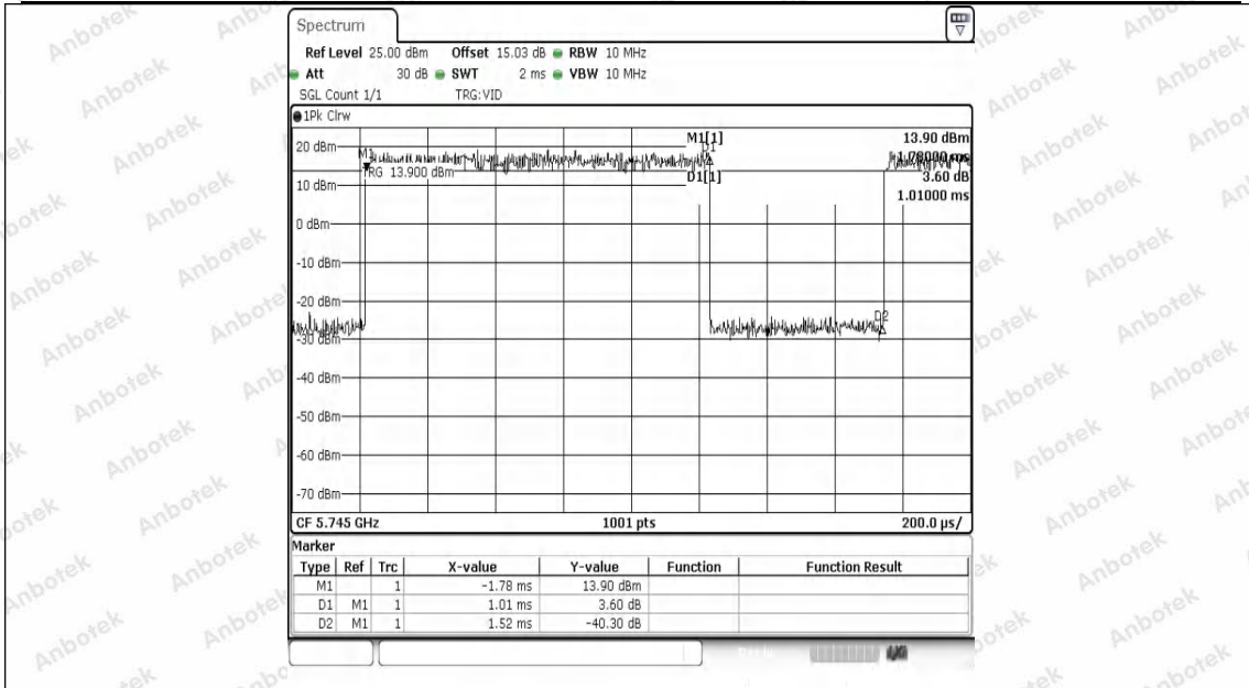
NTNV-11AX20SISO-Ant1-5745
