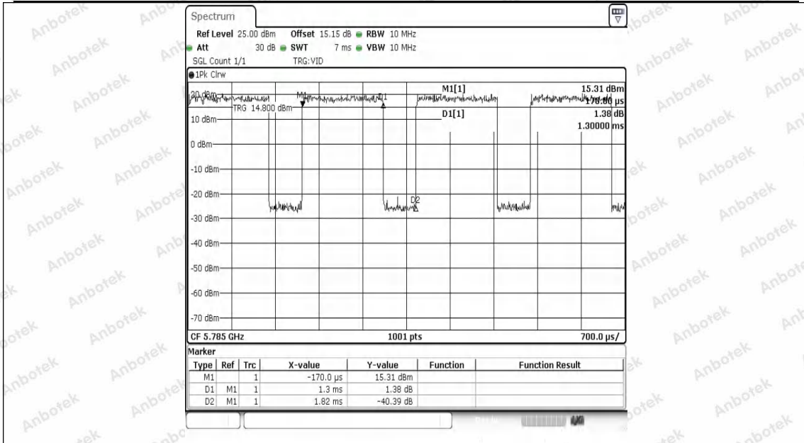
NTVN-11N20SISO-Ant1-5785
