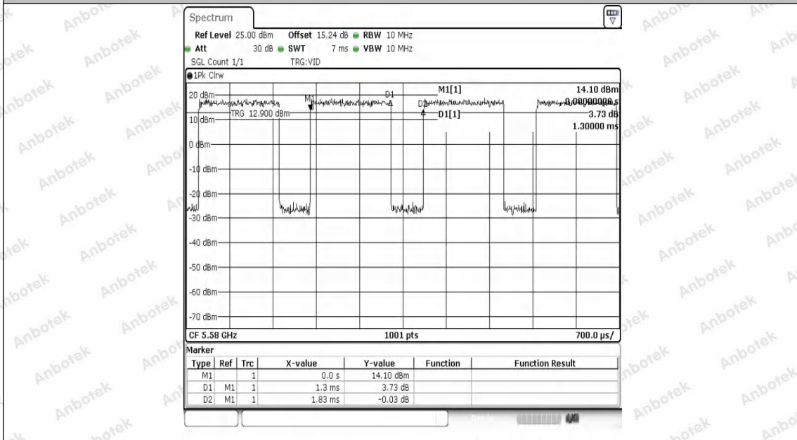
NITNV-11N20SISO-Ant1-5580
