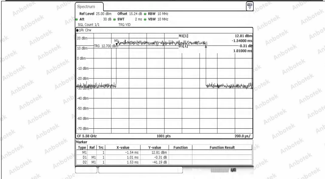
NTNV-11AX20SISO-Ant1-5580
