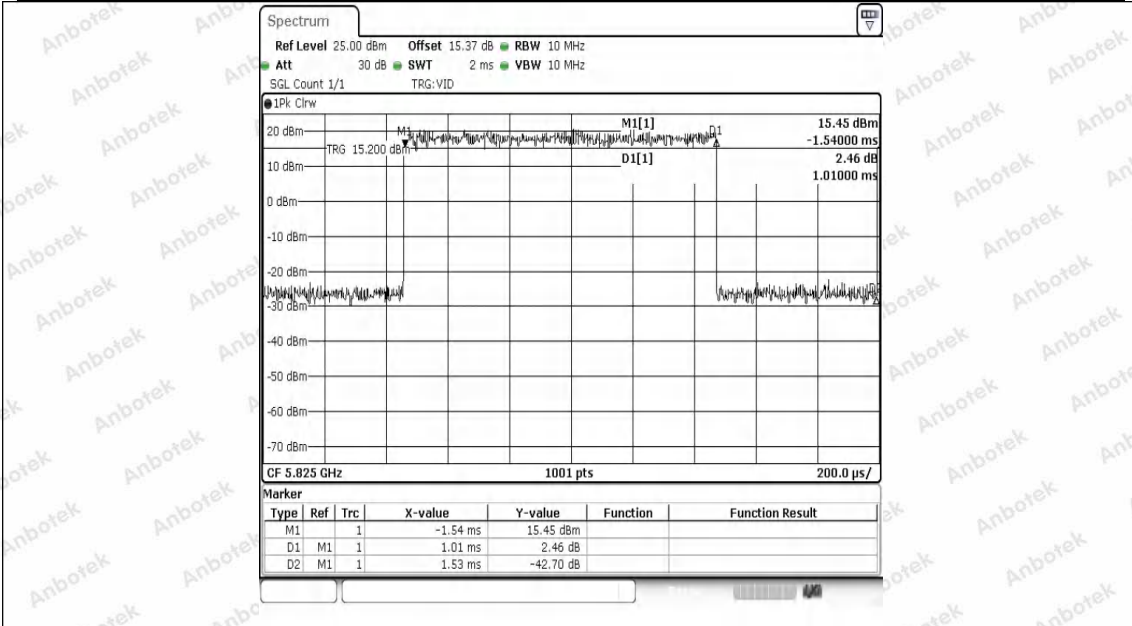
NTNV-11AX20SISO-Ant1-5825
