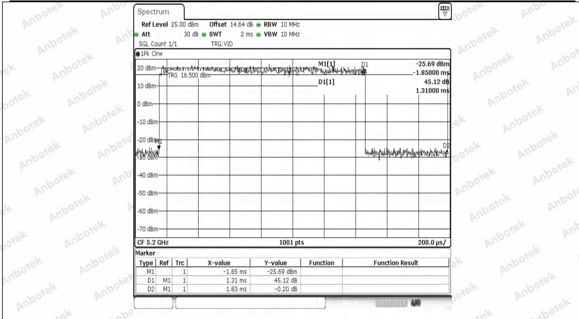
NTNV-11AC20SISO-Ant1-5200
