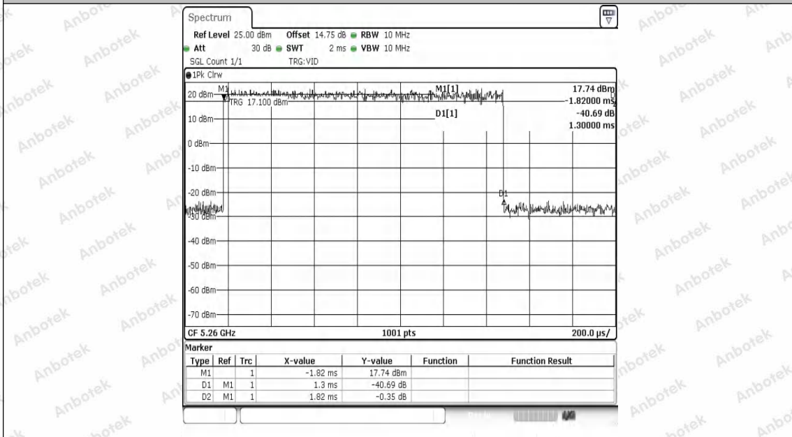
NTVN-11N20SISO-Ant1-5260
