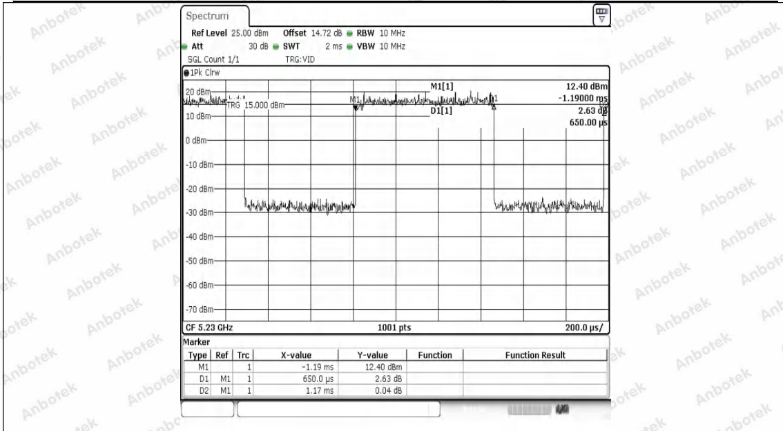
NTNV-11AC40SISO-Ant1-5230
