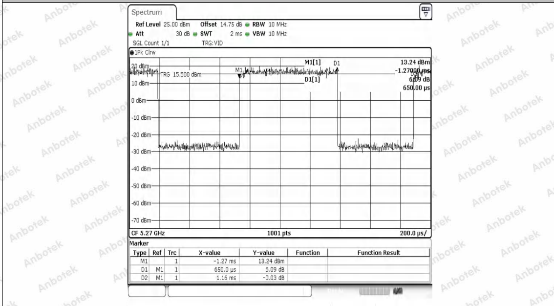
NTNV-11AC40SISO-Ant1-5270
