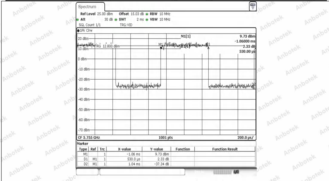
NTNV-11AX40SISO-Ant1-5755
