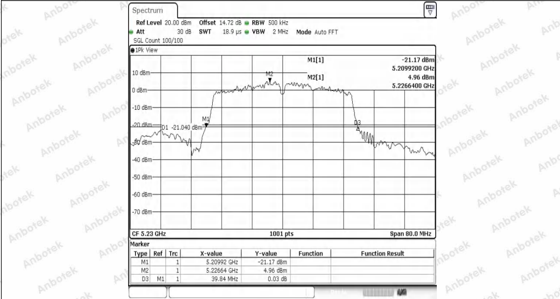
11N40SISO-Ant1-5230
