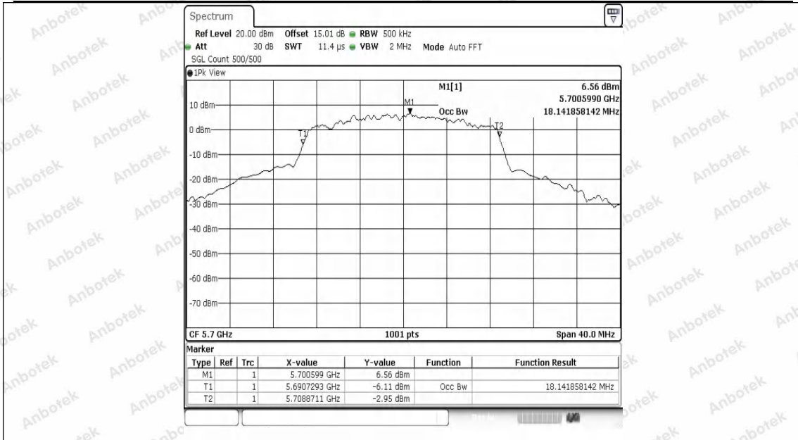
11N20SISO-Ant1-5700
