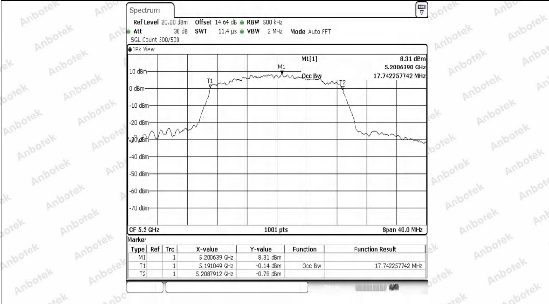
11AC20SISO-Ant1-5200
