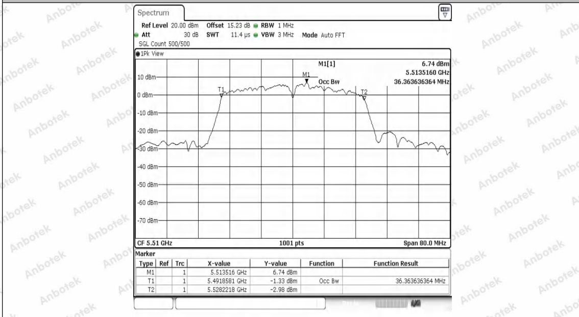
11AC40SISO-Ant1-5510
