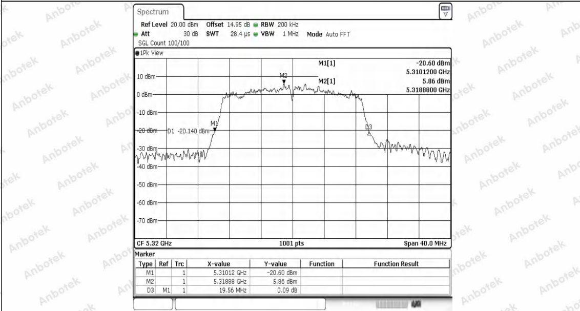
11N20SISO-Ant1-5320
