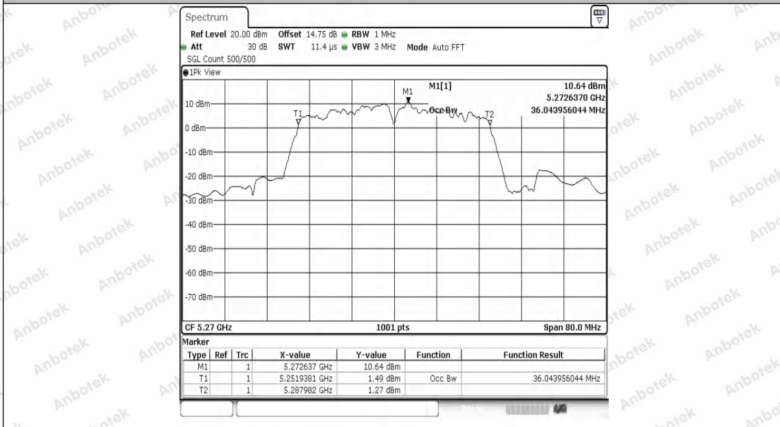
11AC40SISO-Ant1-5270
