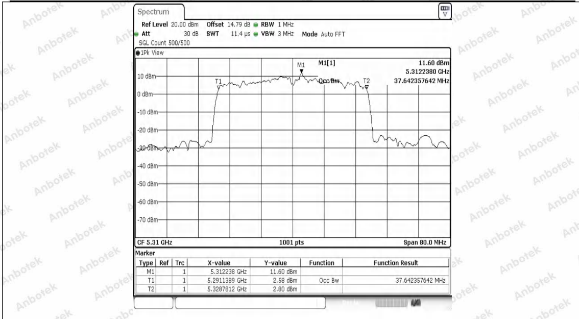
11AX40SISO-Ant1-5310
