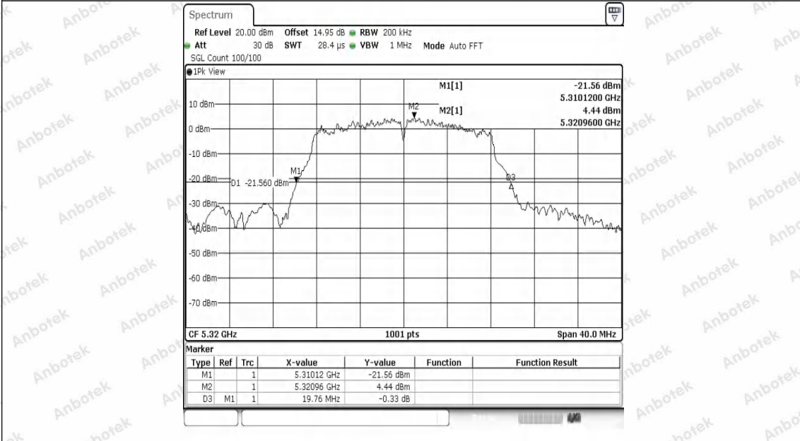
11A-Ant1-5320
