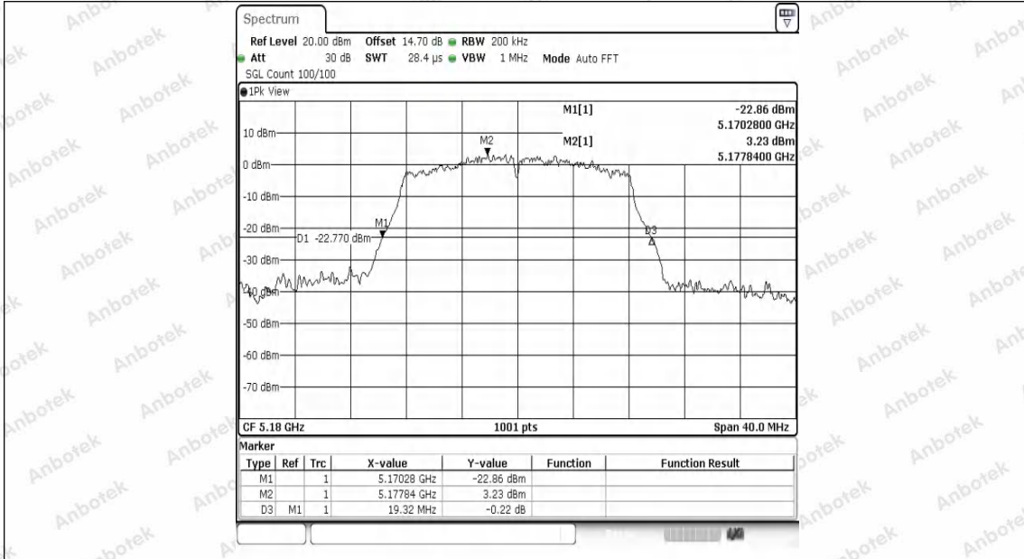
11A-Ant1-5180
