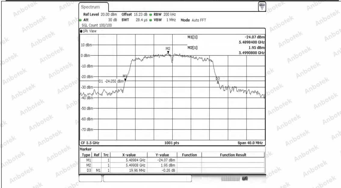
11N20SISO-Ant1-5500
