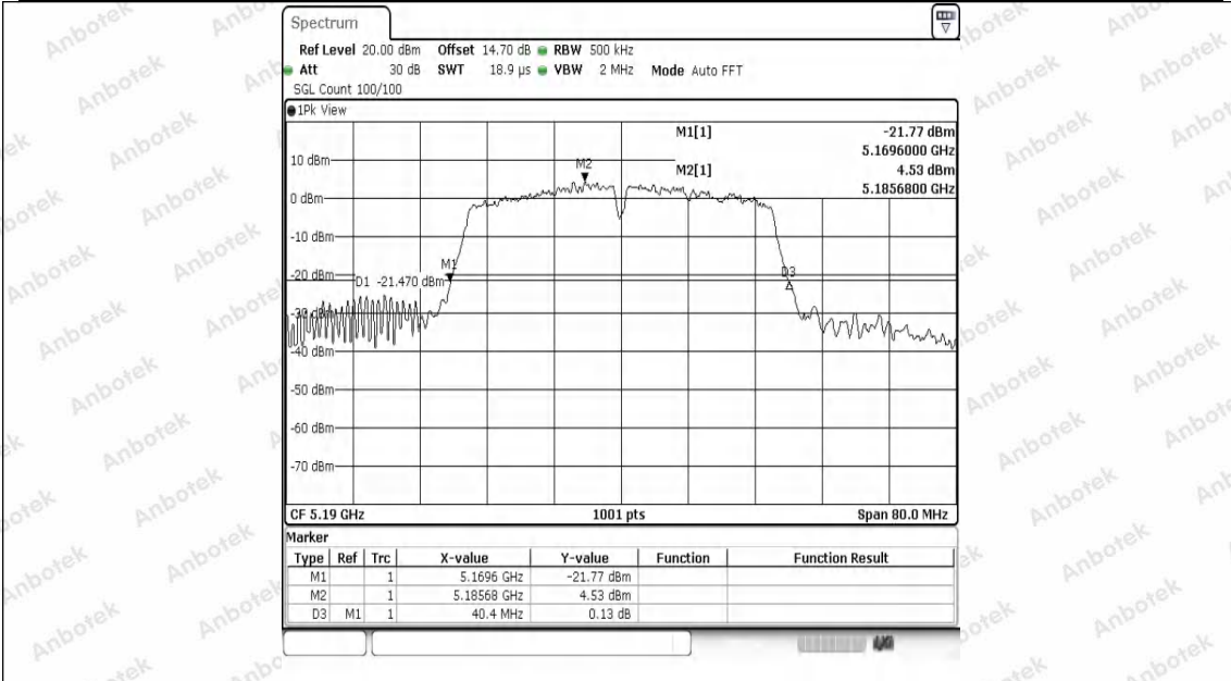
11N40SISO-Ant1-5190
