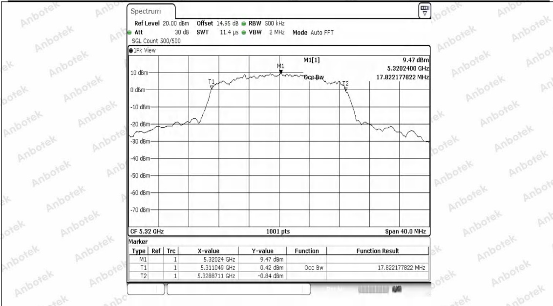
11AC20SISO-Ant1-5320
