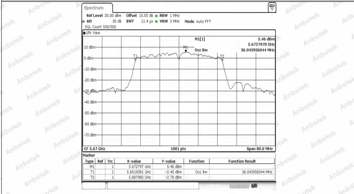
11AC40SISO-Ant1-5670
