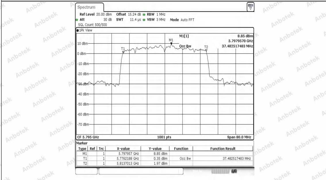
11AX40SISO-Ant1-5795
