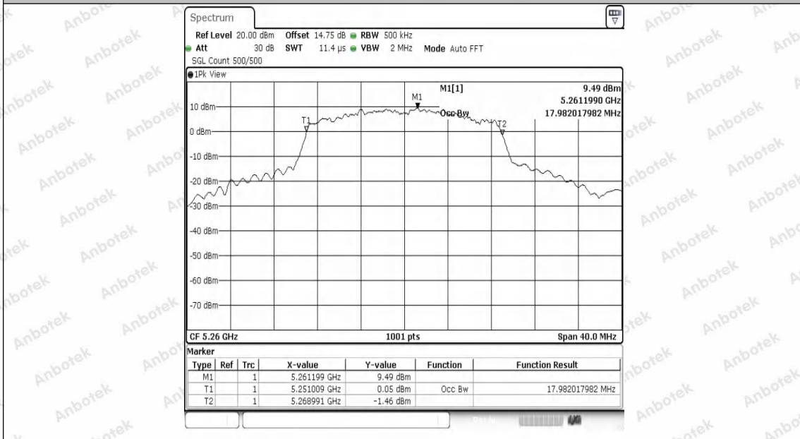
11N20SISO-Ant1-5260
