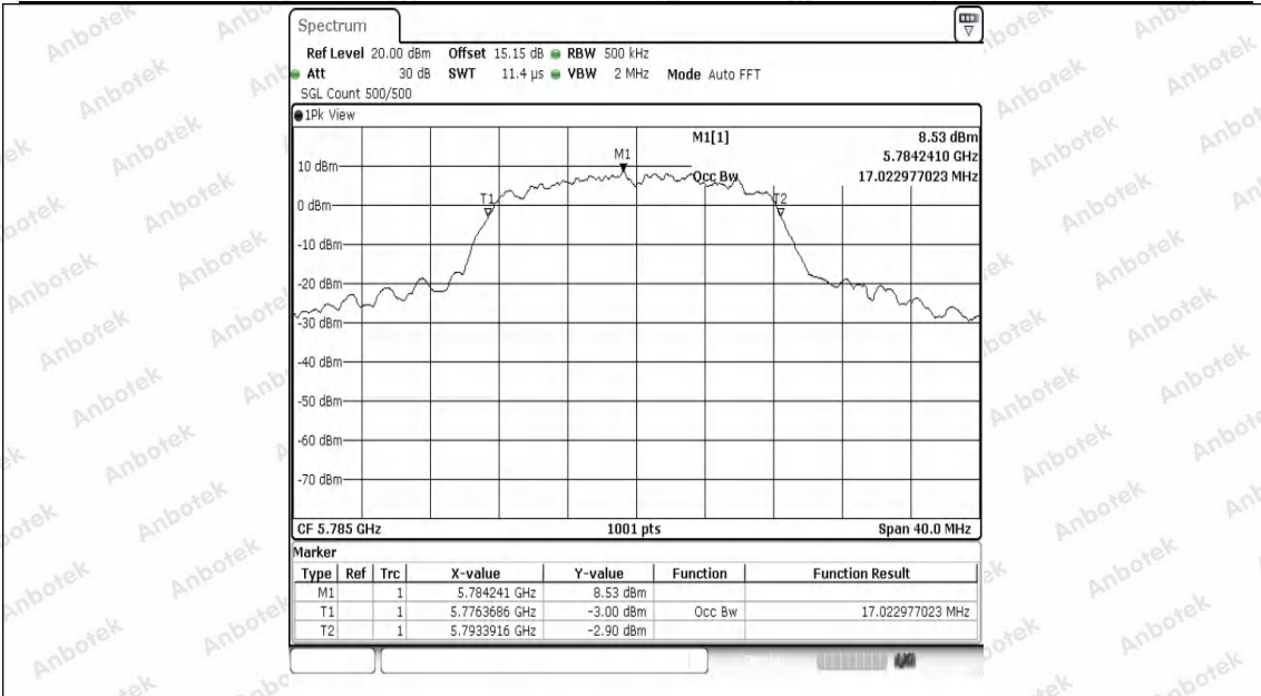
11A-Ant1-5785
