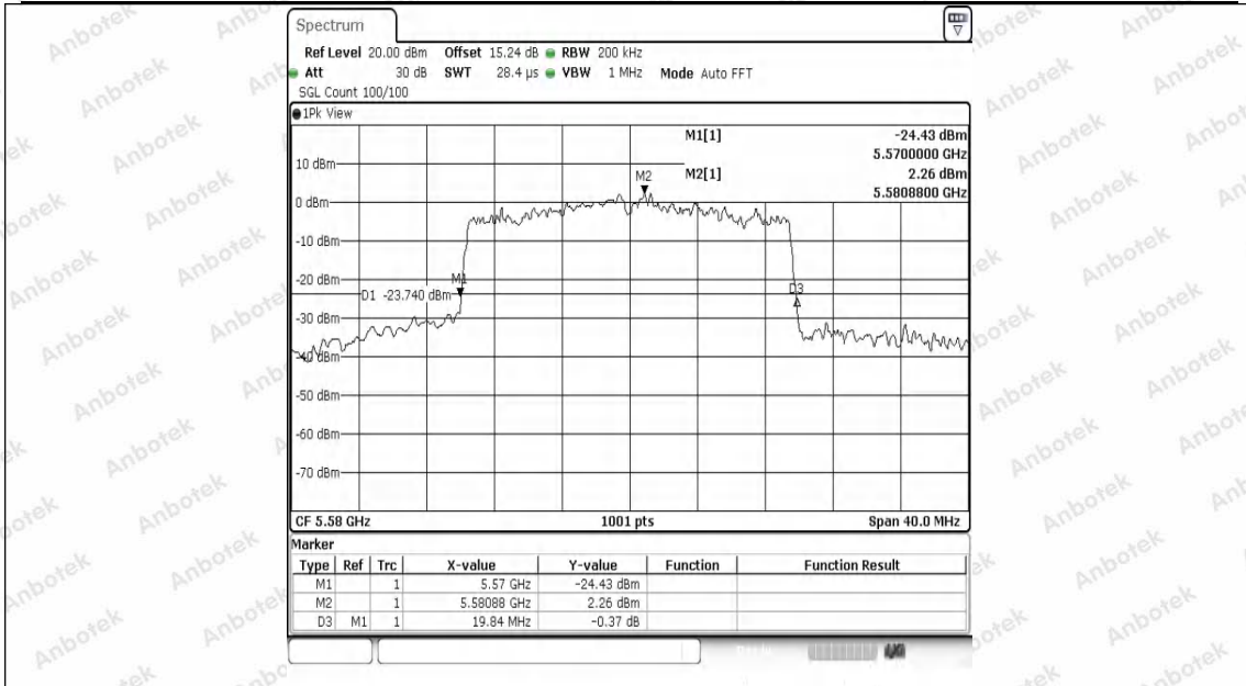
11AX20SISO-Ant1-5580
