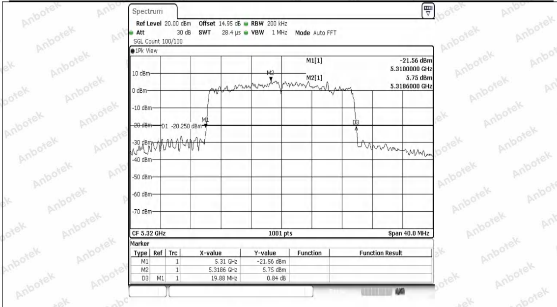
11AX20SISO-Ant1-5320
