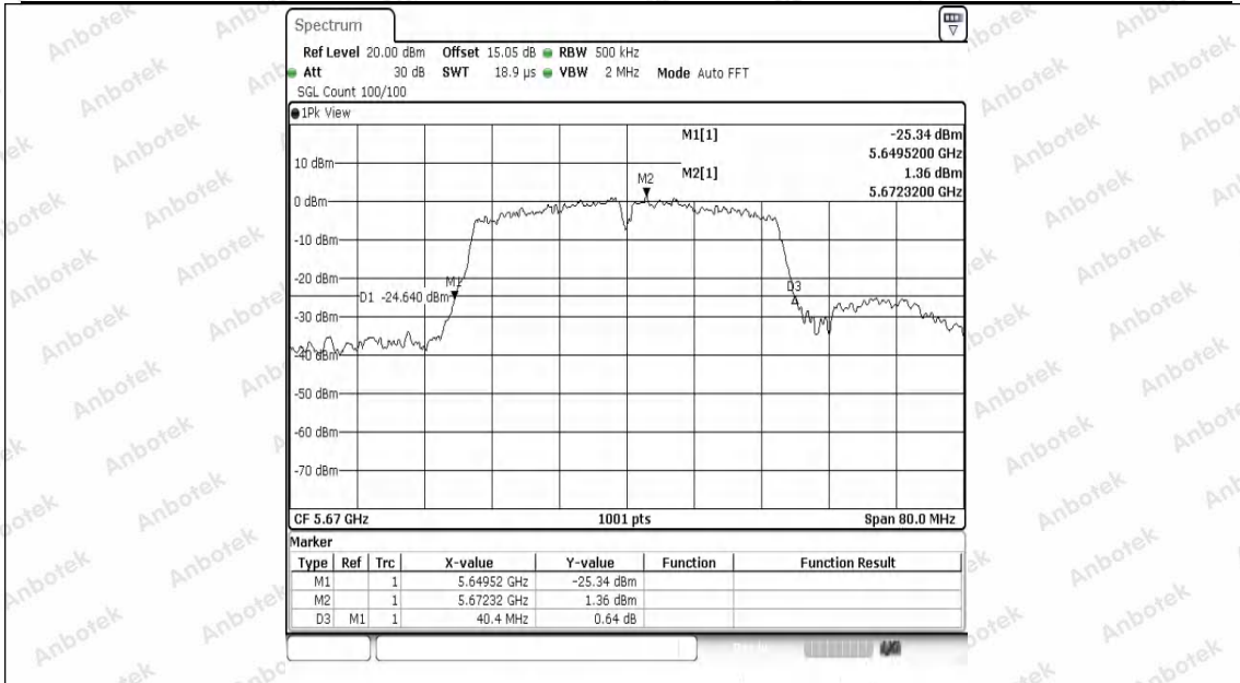
11N40SISO-Ant1-5670
