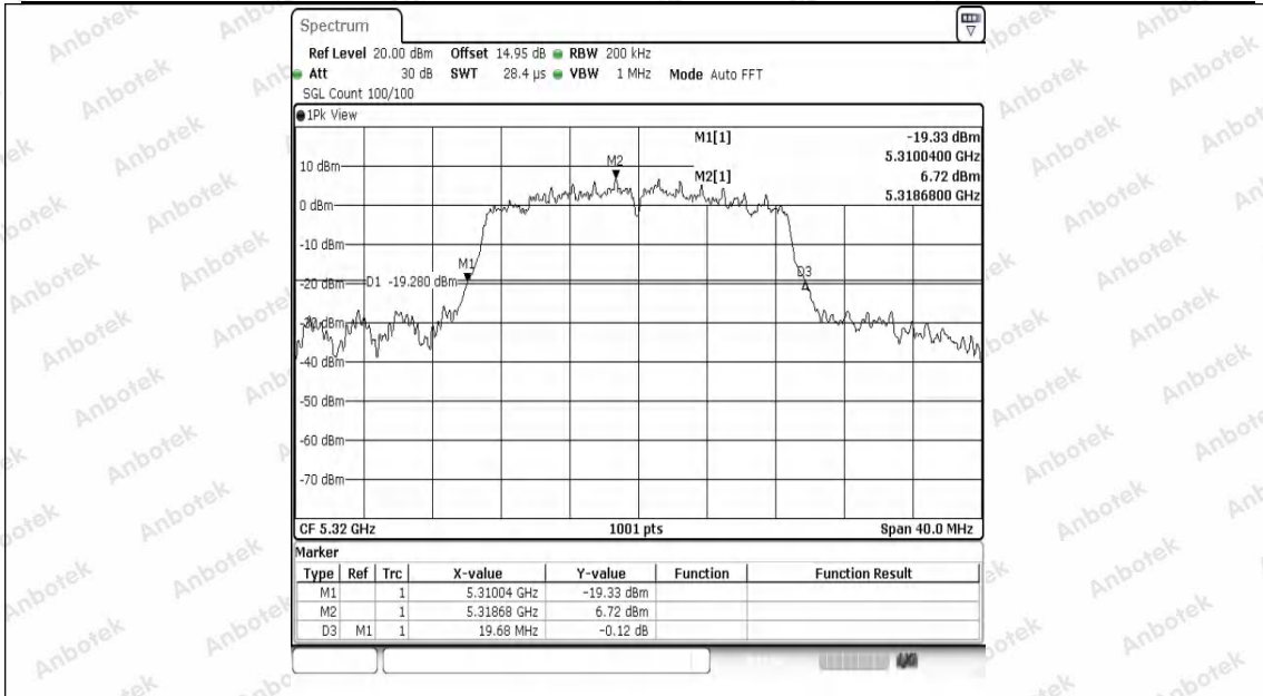
11AC20SISO-Ant1-5320
