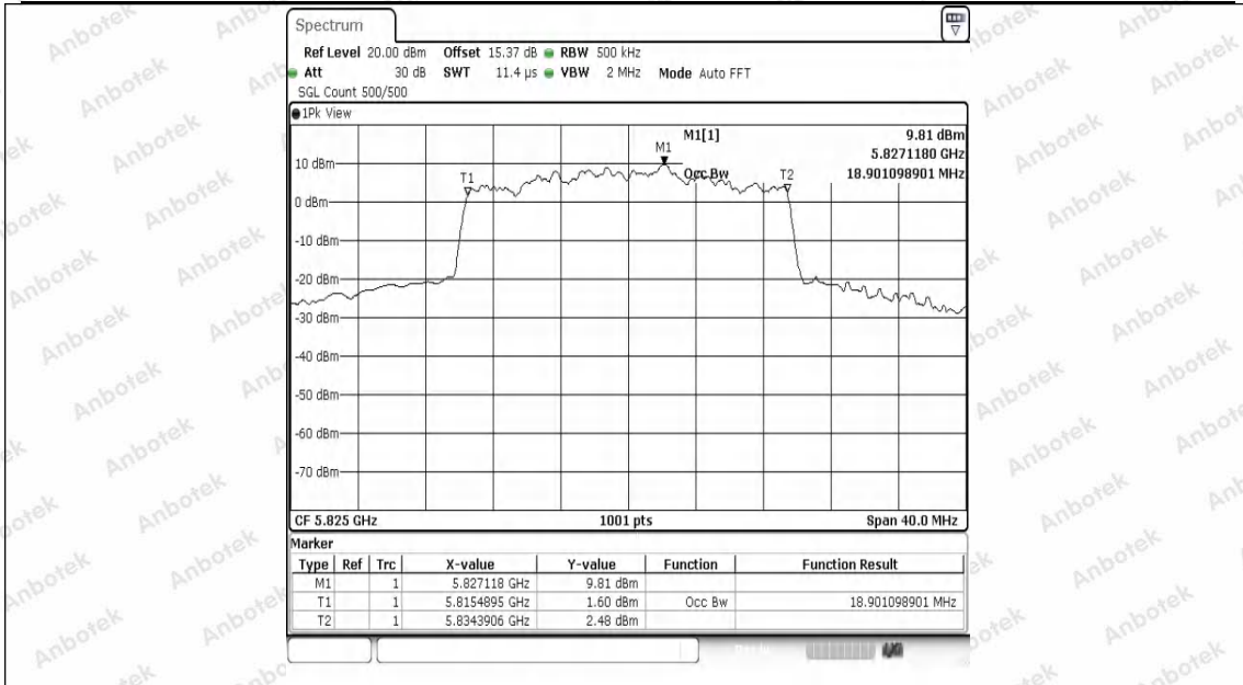
11AX20SISO-Ant1-5825
