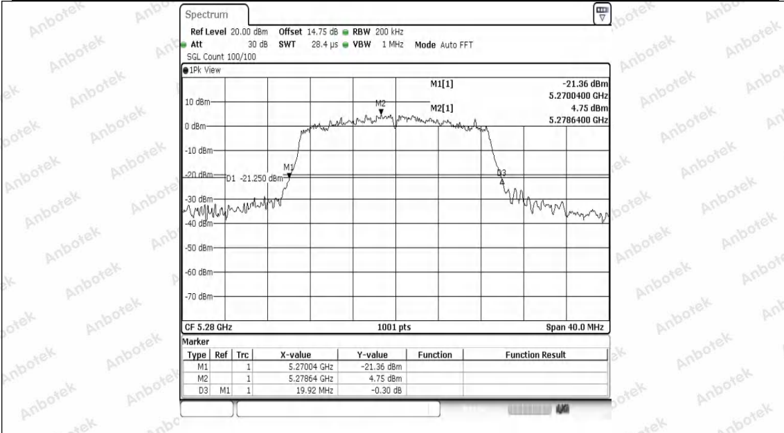
11N20SISO-Ant1-5280
