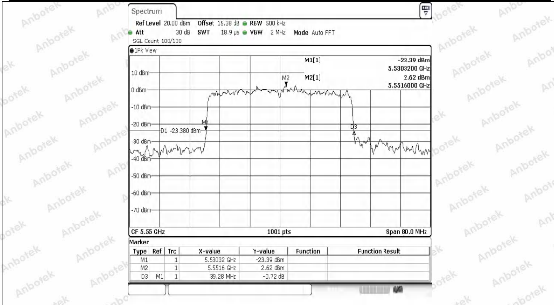
11AX40SISO-Ant1-5550
