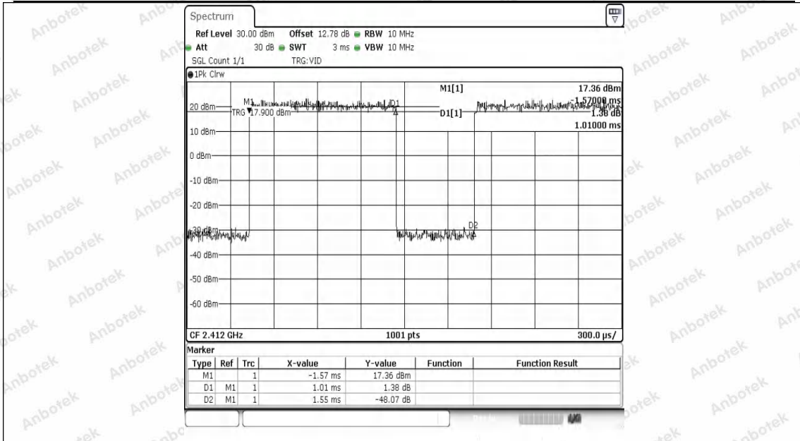
NTNV-11AX20SISO-Ant1-2412
