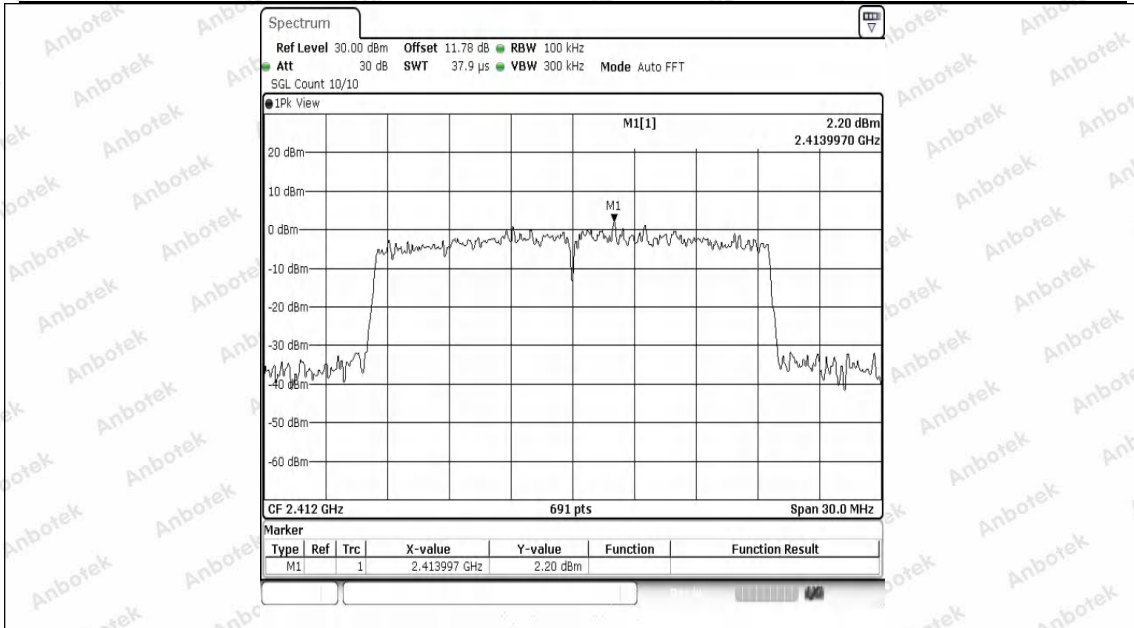
11AX20SISO-Ant1-2412-0~Reference-PASS
