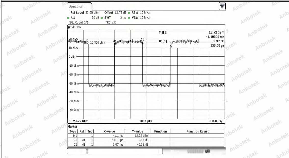
NTVN-11AX40SISO-Ant1-2422
