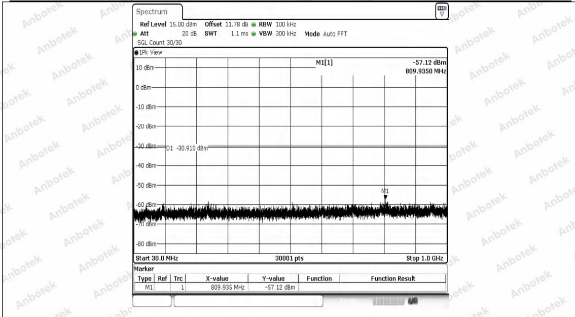
11AX40SISO-Ant1-2422-30~1000-PASS
