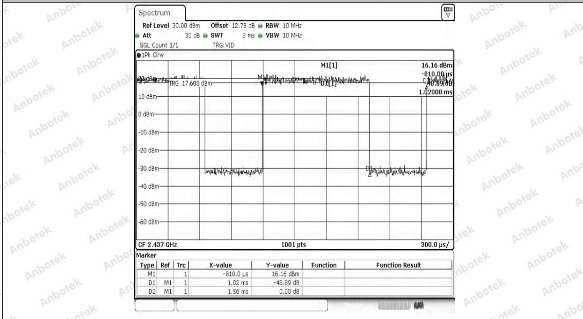
NTNV-11AX20SISO-Ant1-2437
