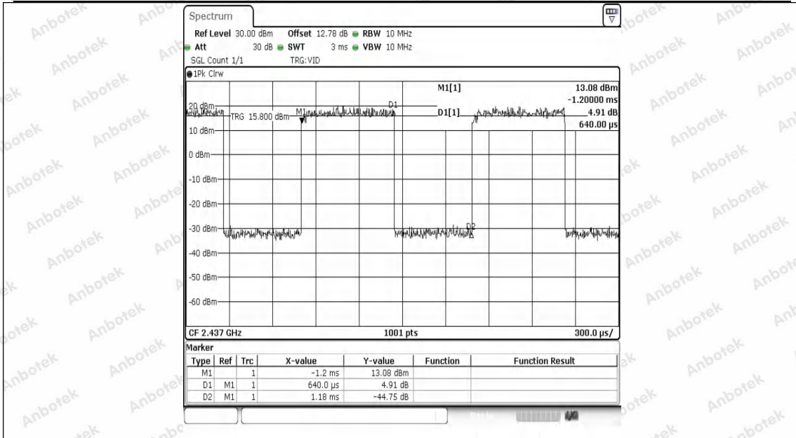
NTVN-11N40SISO-Ant1-2437
