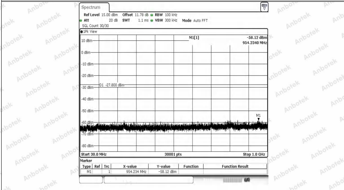
11AX20SISO-Ant1-2412-30~1000-PASS
