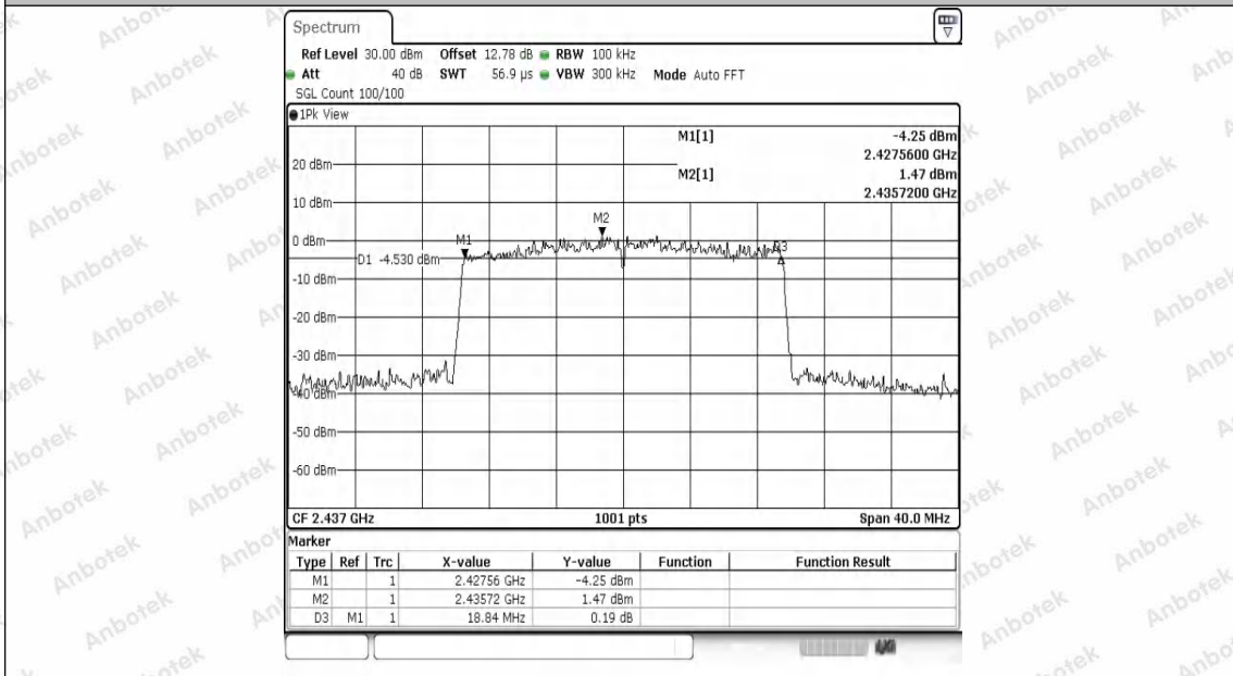
11AX20SISO-Ant1-2437-PASS
